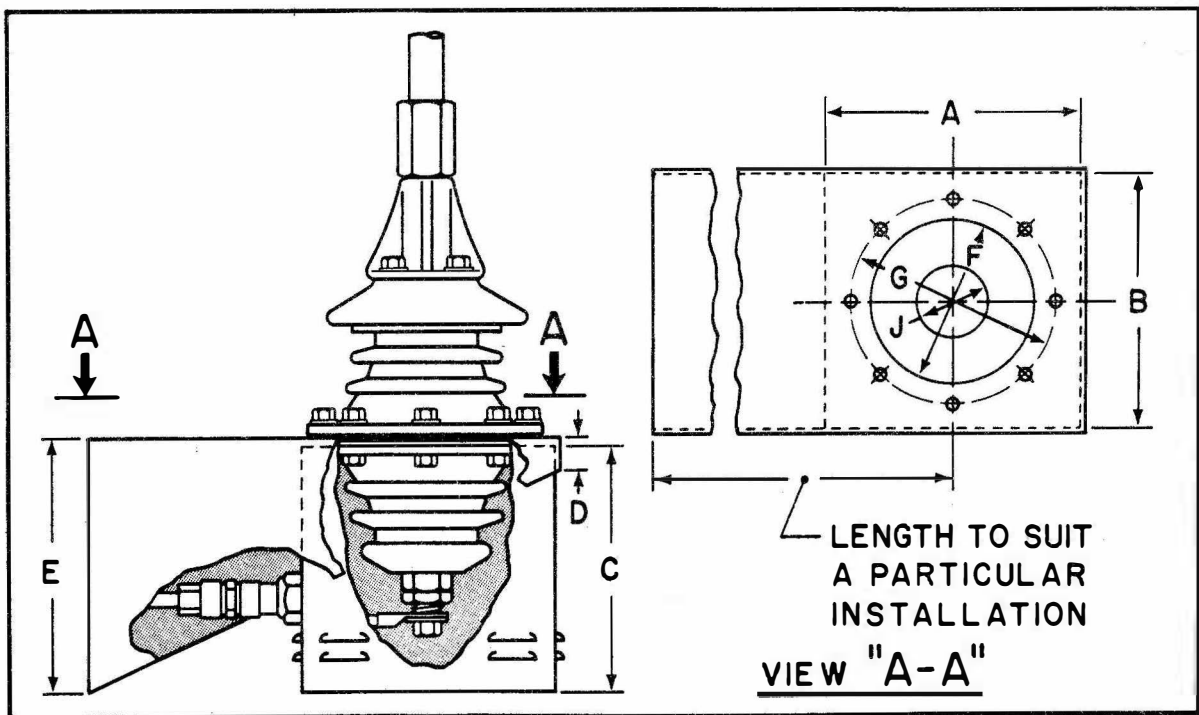
Figure 4-1. Stationary Whip.
