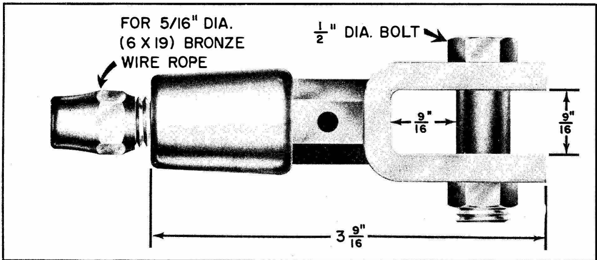
Figure 3-7. MX-1178/U Connector.
