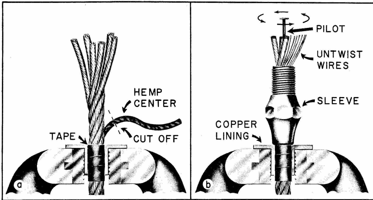
Figure 3-8. MX-1178/U Installation Details.
