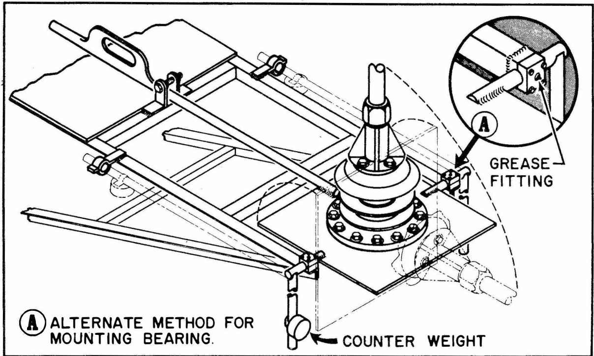
Figure 4-2. Tilting Whip.
