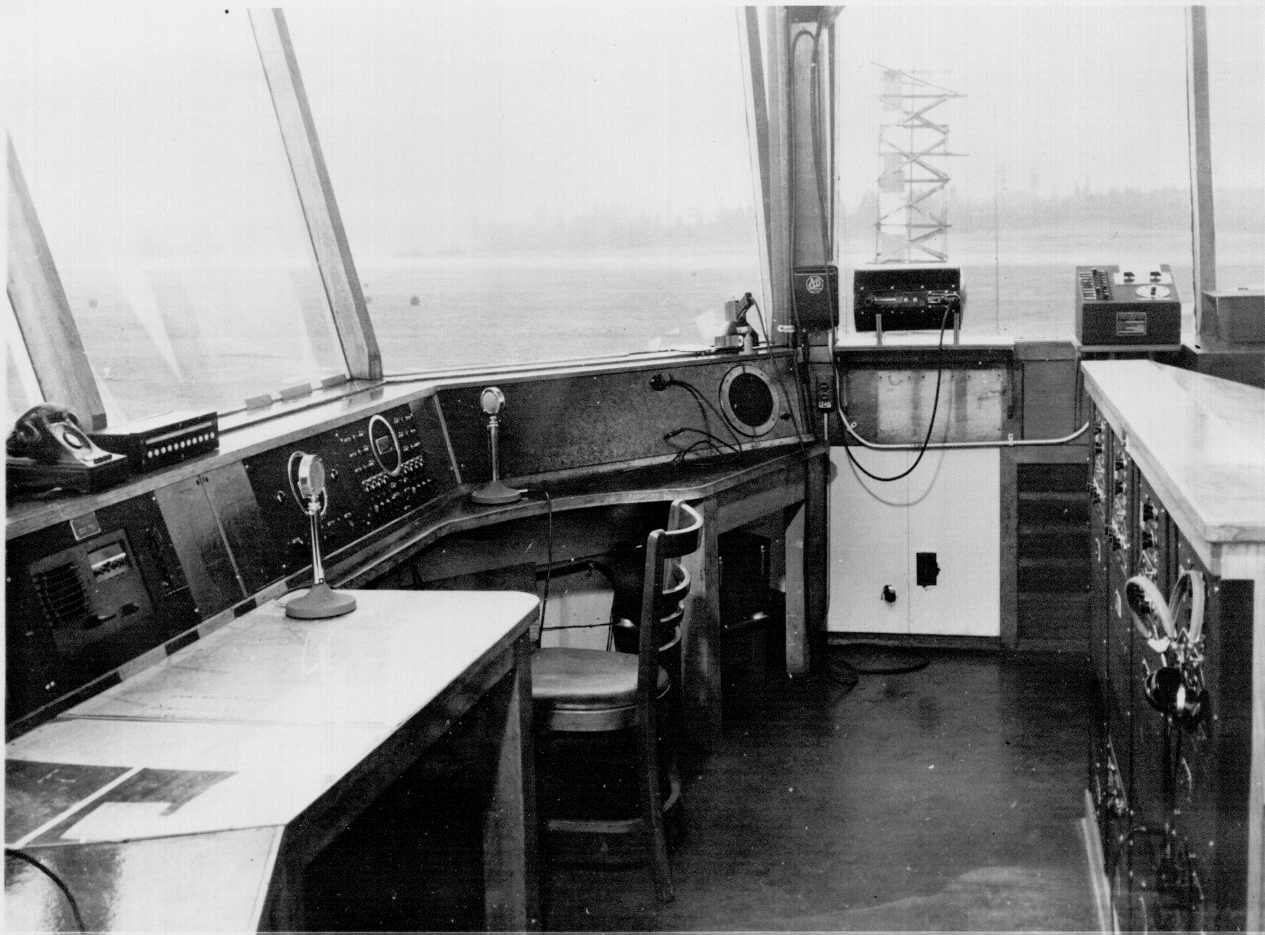
2505-45 Puget Sound Navy Yard 15 May 1945 Photograph (A) Typical Control Desk Installation.
