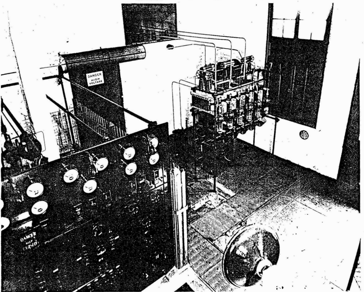
80/100 KW transmitter - Chollas Heights. MO, control panels & rectifier.
