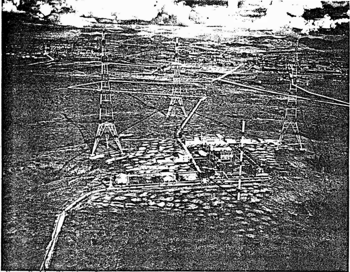
Navy Radio Station Chollas Heights - from 600 feet - looking east 1935
