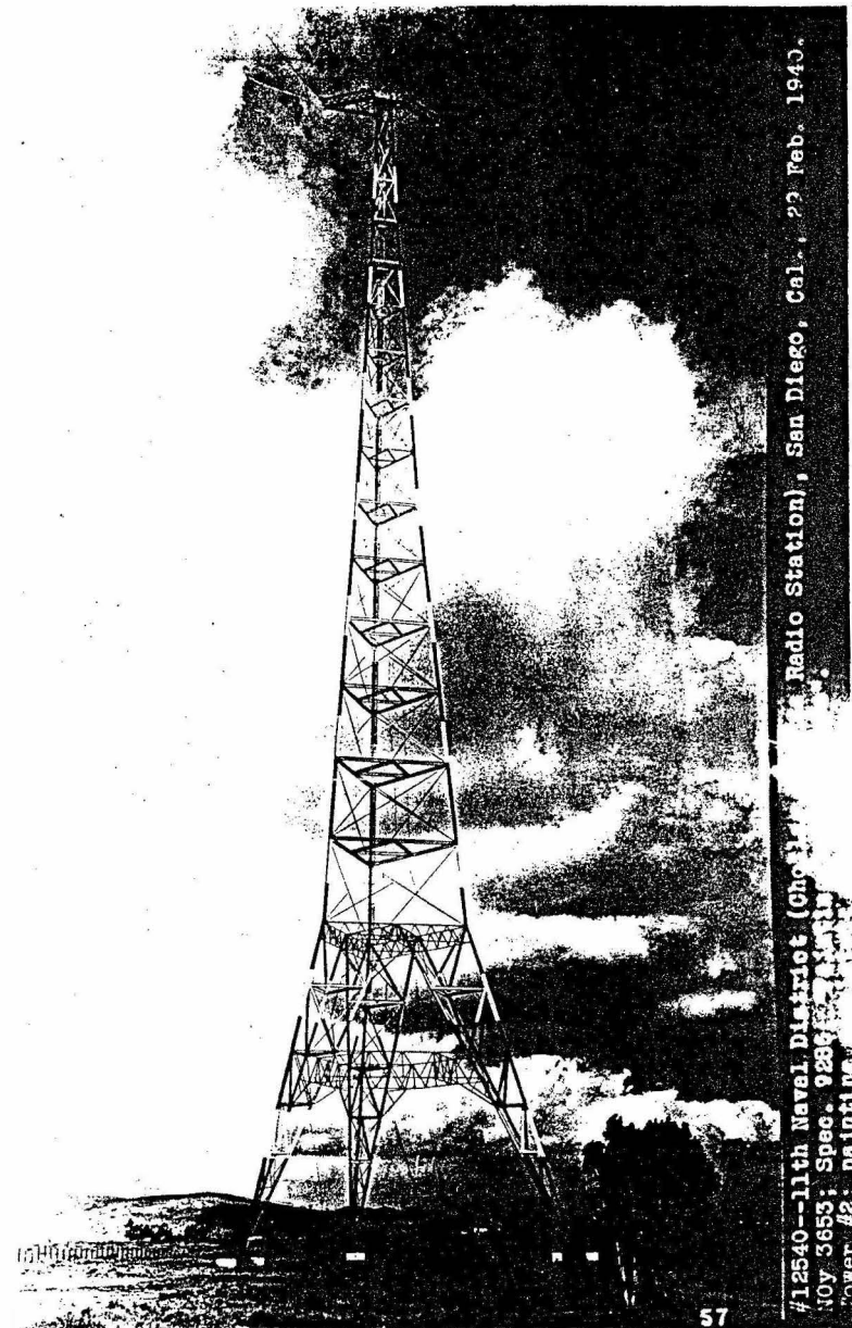
One of three 600 foot steel towers -Chollas Heights
