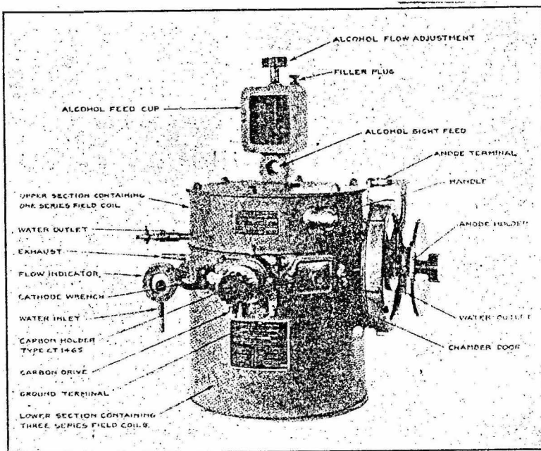
2kw Arc Transmitter
