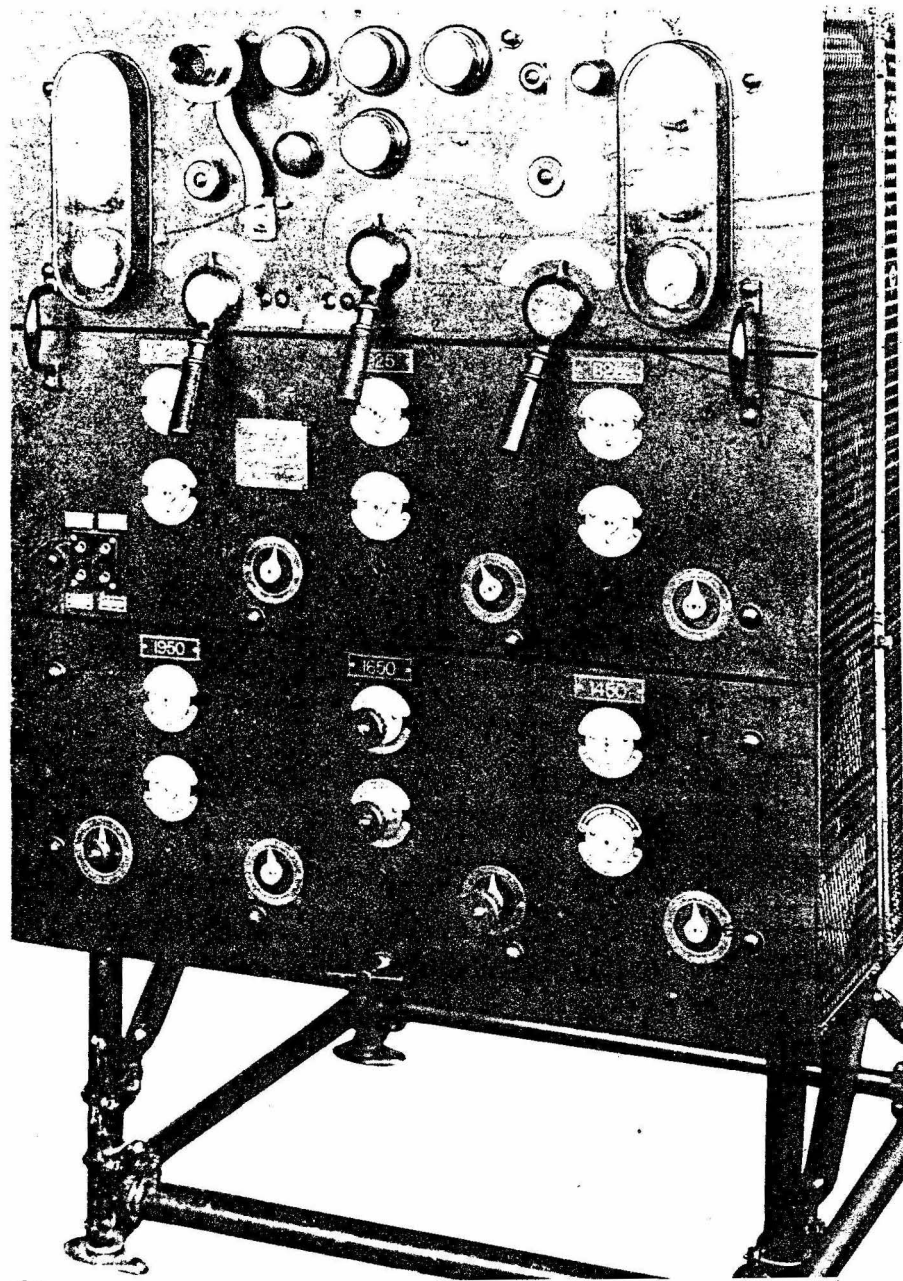
Navy Model "TA" Transmitter at NFL, foot of Broadway, 1923. Antenna was a 6 strand flat-top between Navy Headquarters building and the stacks on the Kettner Powerhouse. The transmitter nameplate stated it had been built by Westinghouse for the Venezuela Government - but it was bought by the Navy as the first vacuum tube transmitter - the "TA."
