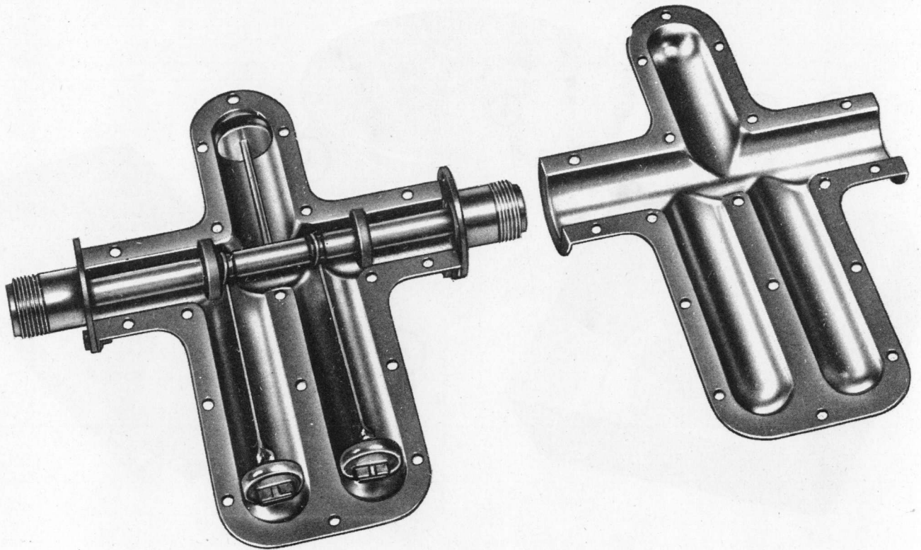
Figure 6-40. Wave Trap F-41/SPR-1, Open View.
