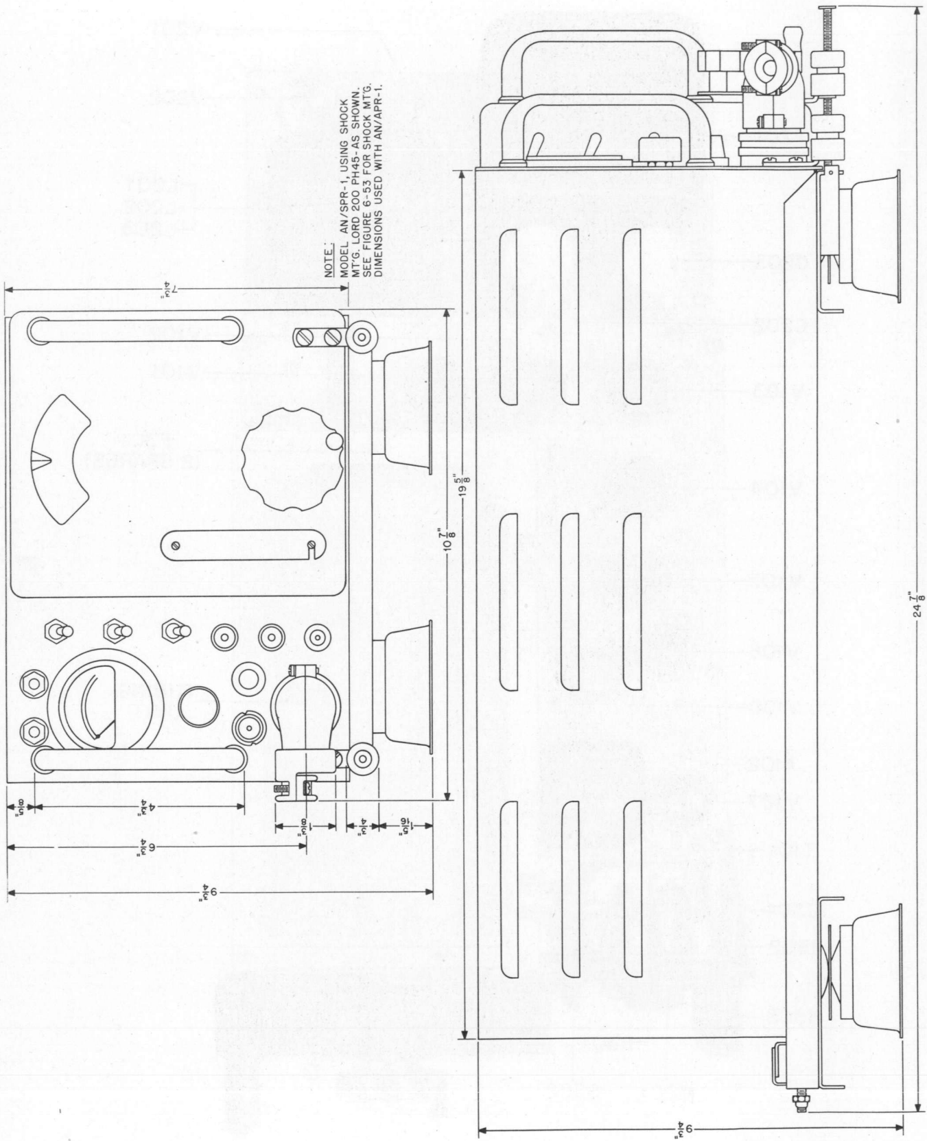
Figure 6-52. Radio Receiving Equipment AN/APR-1 and AN/SPR-1, Overall Dimensional.
