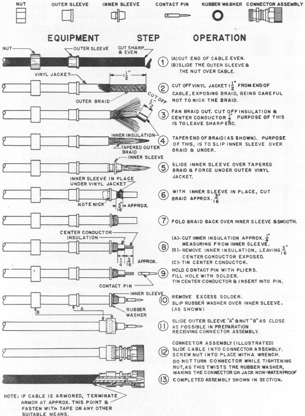
Figure 6-69. Connector Assembly.
