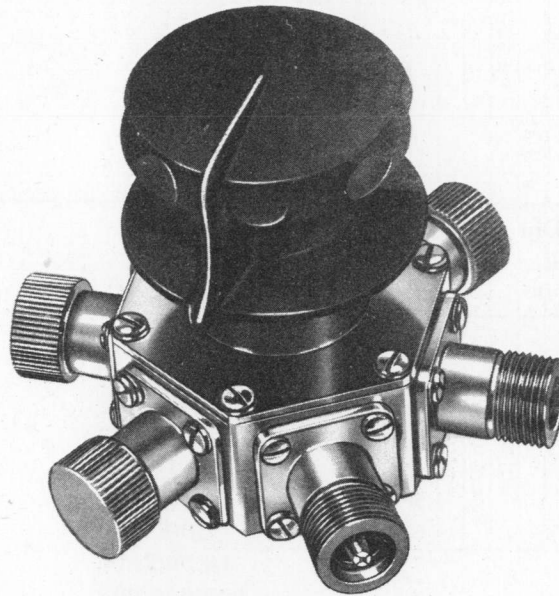
Figure 6-77. R. F. Switch SA-44(A)/APR, Top View.
