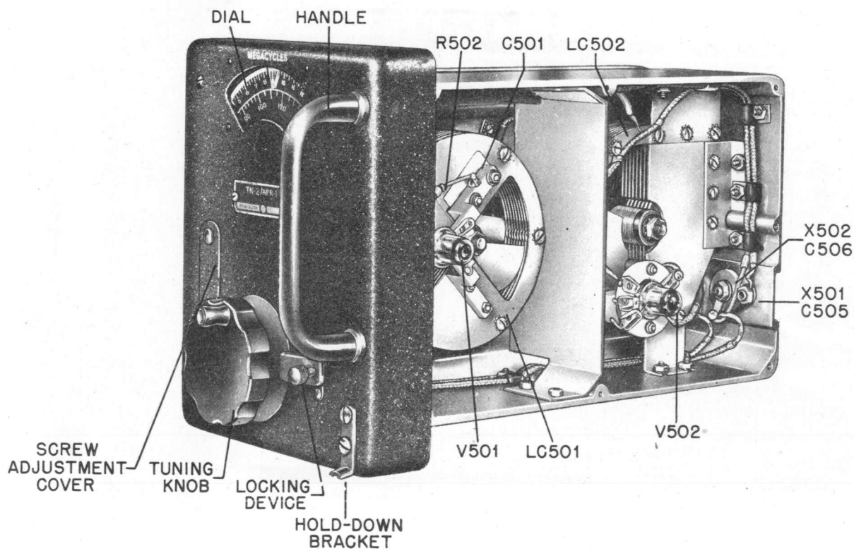
Figure 6-8. Tuning Unit TN-2/APR-1, Right Front Oblique View.
