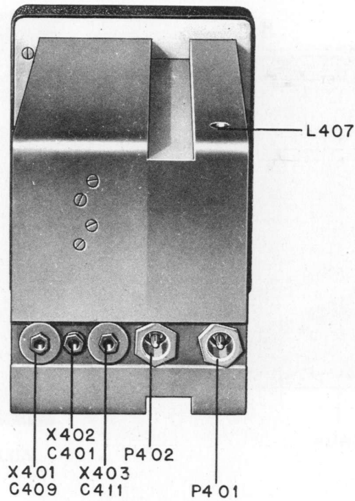
Figure 6-18. Tuning Unit TN-3/APR-1, Rear View.
