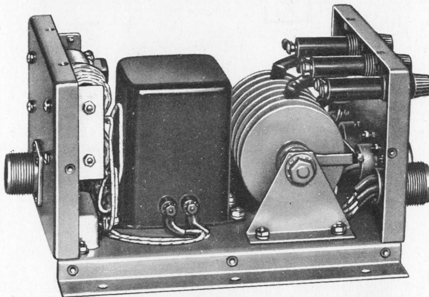
Figure 6-26. Rectifier Filter Unit PP-183/SPR-1, Left Oblique.
