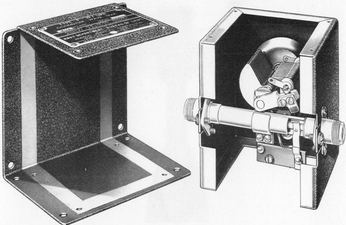
Figure 6-29. Wave Trap F-19/UPR, Open View.
