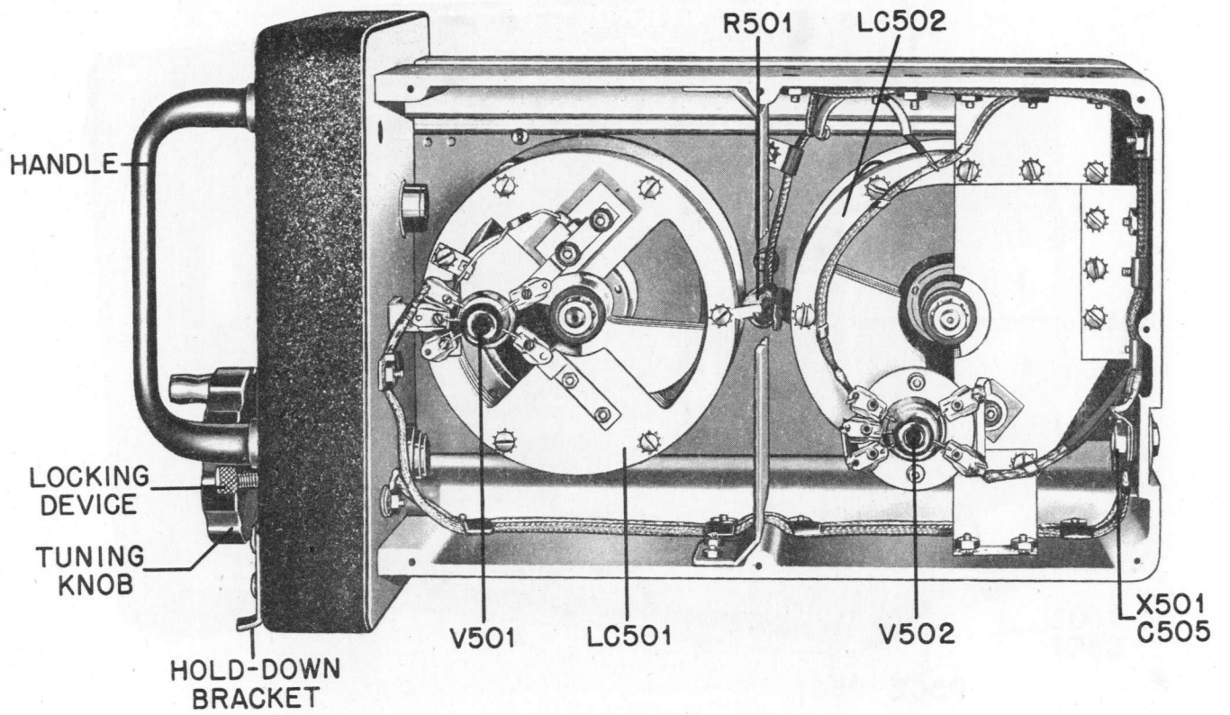
Figure 6-9. Tuning Unit TN-2/APR-1, Right Side View.
