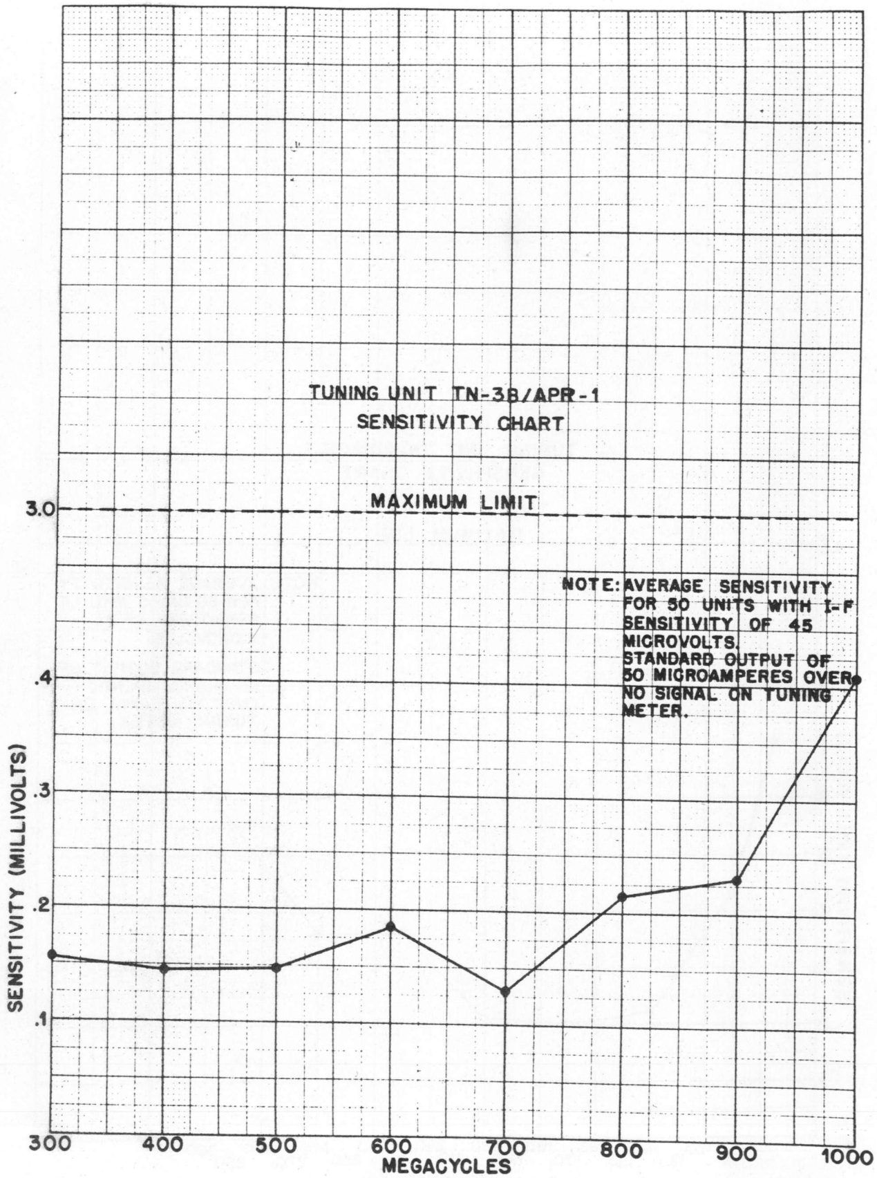
Figure 6-66. Tuning Unit TN-3B/APR-1 Sensitivity Chart.
