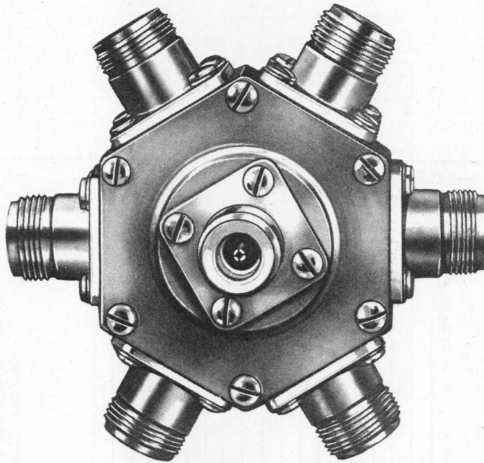
Figure 6-78. R. F. Switch SA-44(A)/APR, Bottom View.
