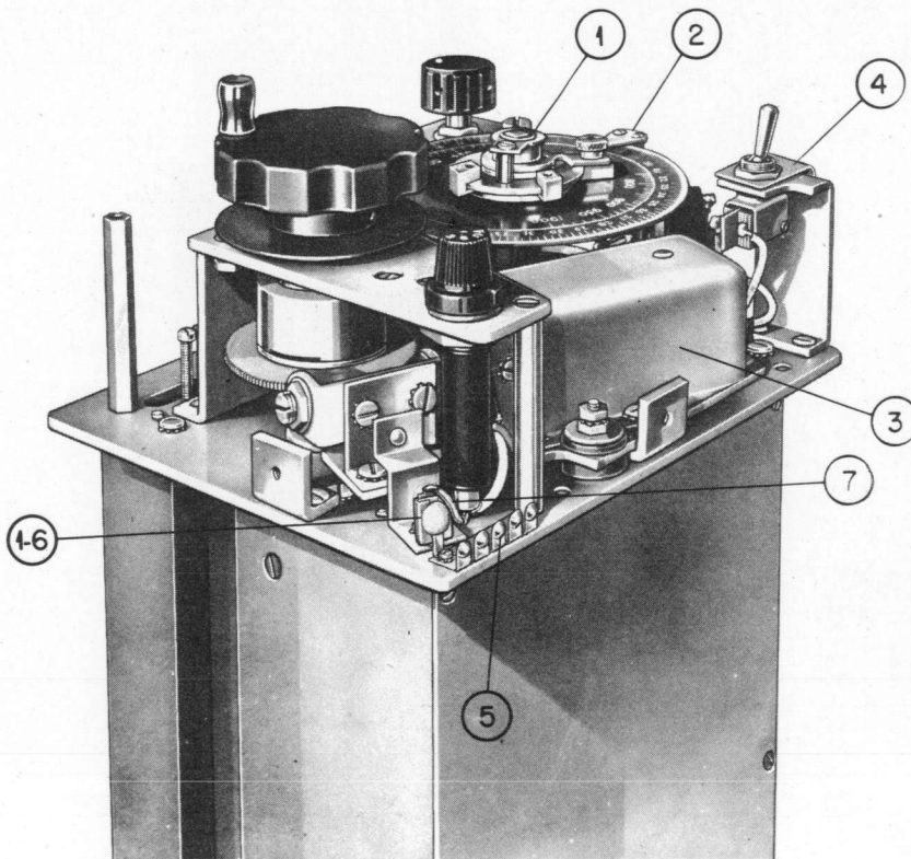
Figure 6-44. Sector Sweep, Top Panel.
