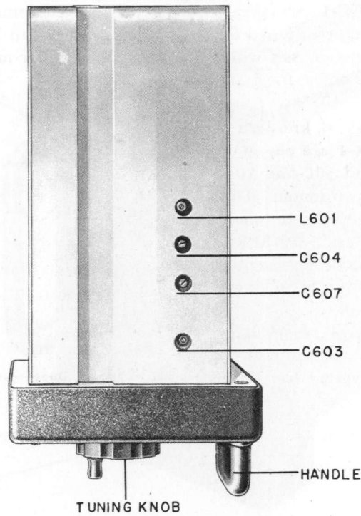
Figure 6-1. Tuning Unit TN-1/APR-1, Top View.
