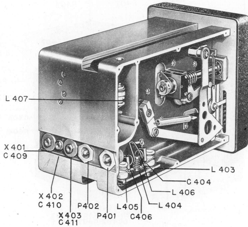
Figure 6-17. Tuning Unit TN-3/APR-1, Rear Left Oblique View.
