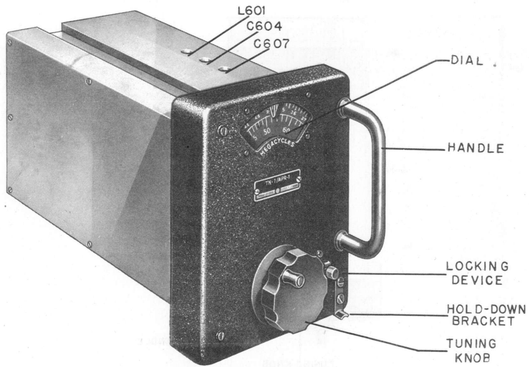
Figure 6-3. Tuning Unit TN-1/APR-1, Left Front Oblique View.
