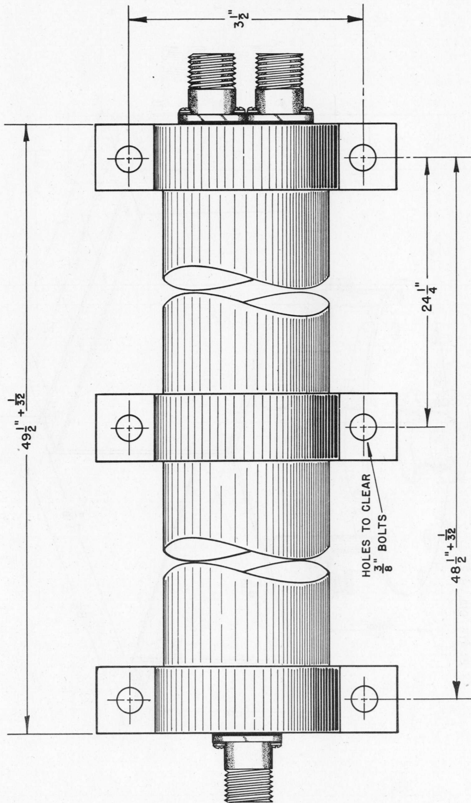
Figure 6-61. Impedance Matching Transformer CU-19/SPR-1, Outline Dimensional.
