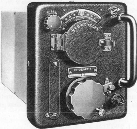
Figure 1-11. Sector Sweep Tuner, Front Panel.
