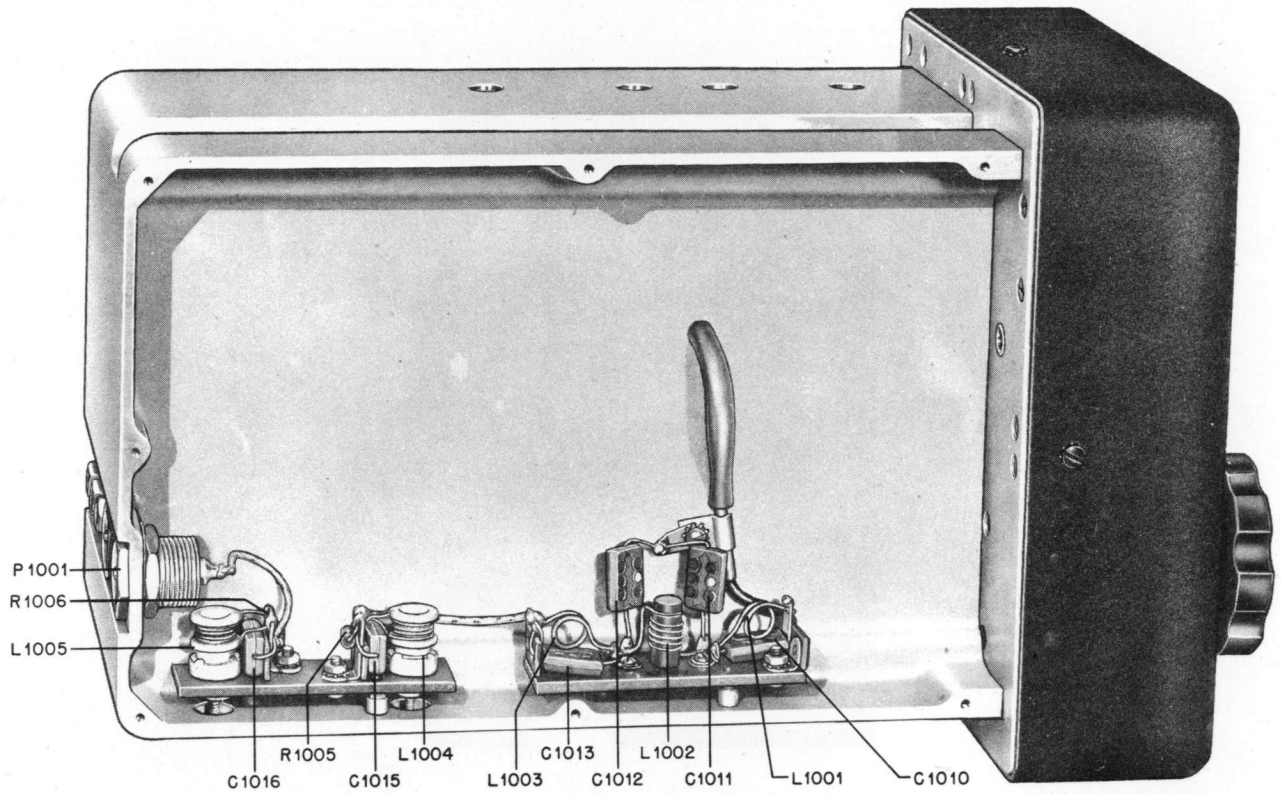
Figure 6-2. Tuning Unit TN-1B/APR-1, Left Side View.
