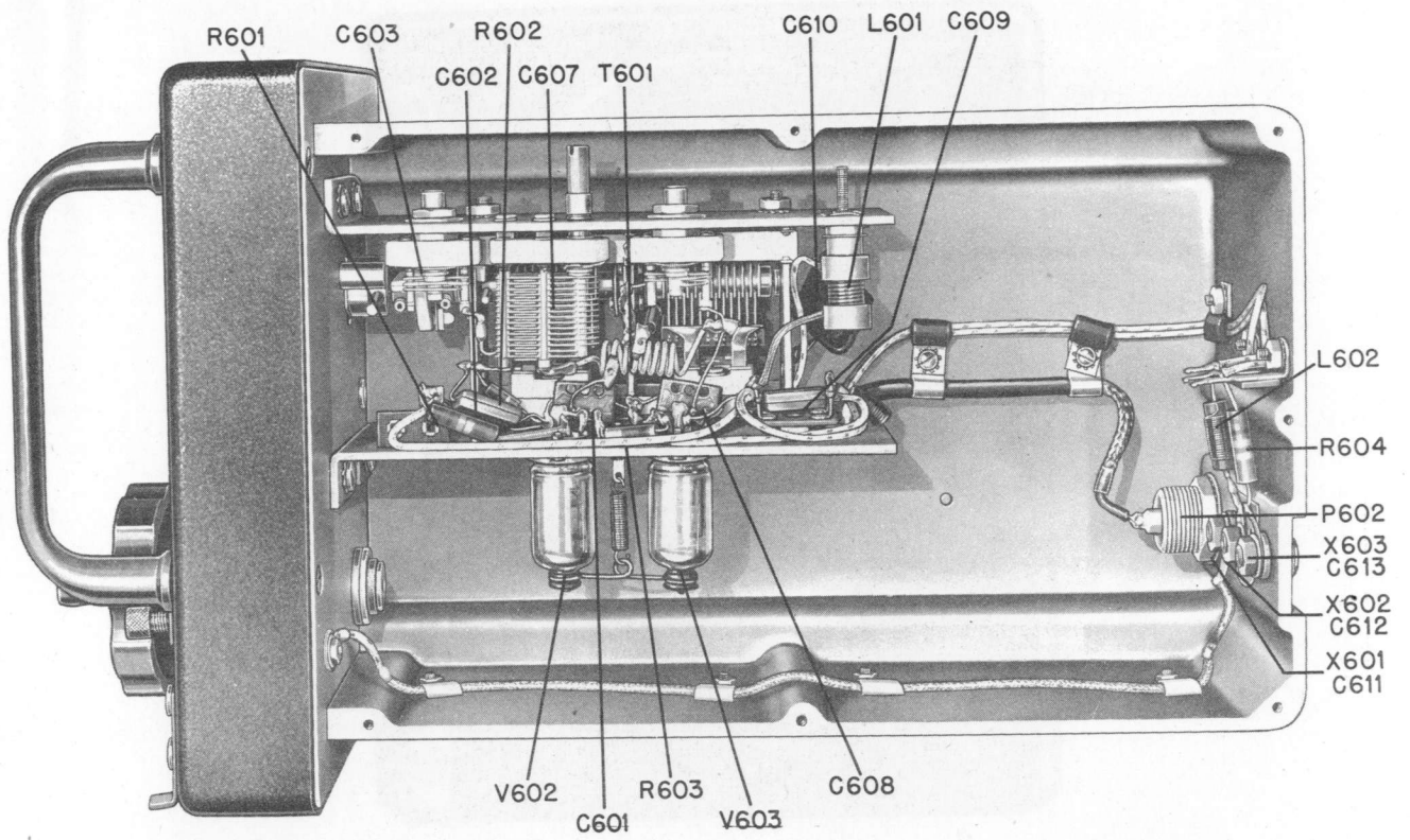
Figure 6-5. Tuning Unit TN-1/APR-1, Right Side View.
