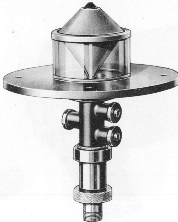
Figure 6-39. Cone Antenna AS-44/APR-5.
