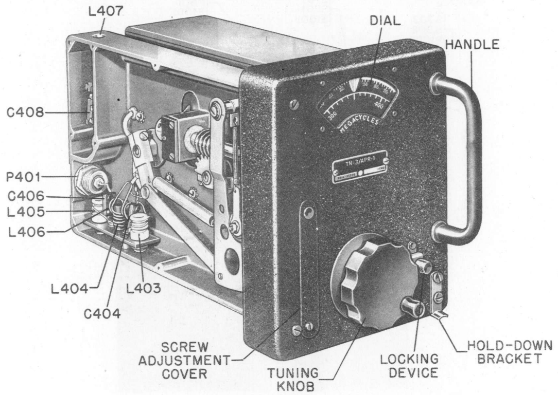
Figure 6-21. Tuning Unit TN-3/APR-1, Front Left Oblique View.
