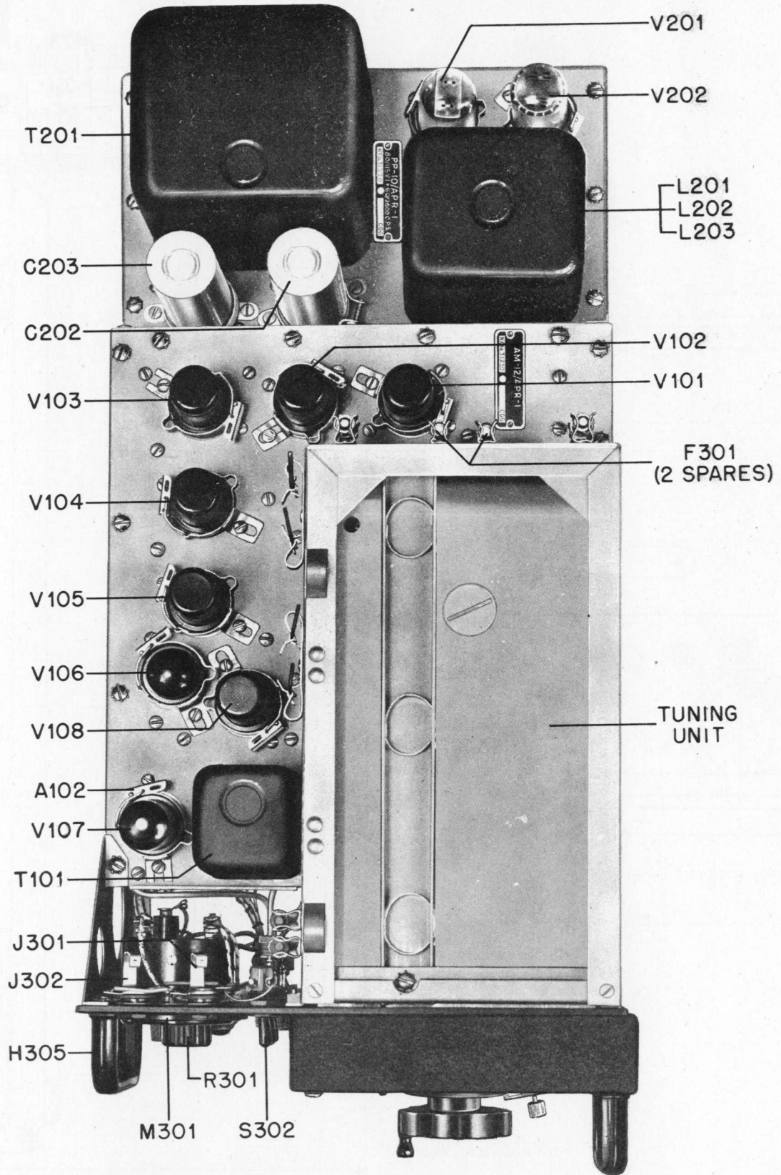
Figure 6-51. Amplifier Strip AM-12/APR-1, Rectifier PP-10/APR-1 and Tuning Unit, Top View.
