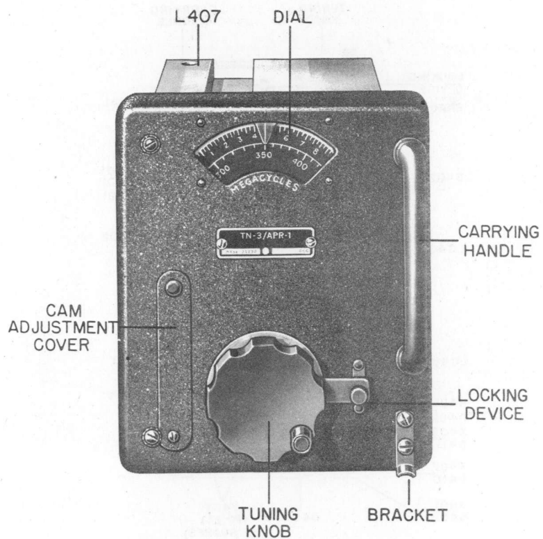
Figure 6-14. Tuning Unit TN-3/APR-1, Front View.
