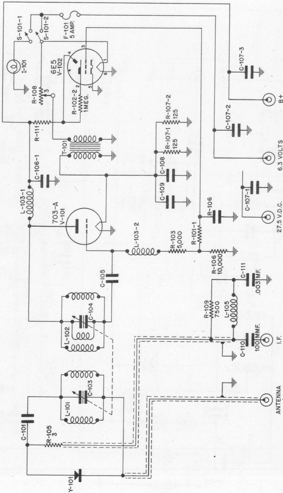
Figure 8-11. Tuning Unit TN-4/APR-1, Schematic.
