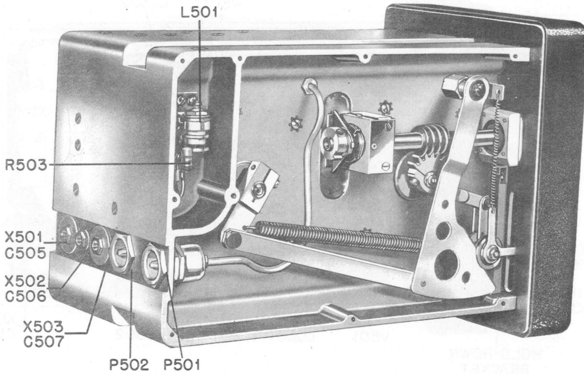
Figure 6-11. Tuning Unit TN-2/APR-1, Rear Right Oblique View.
