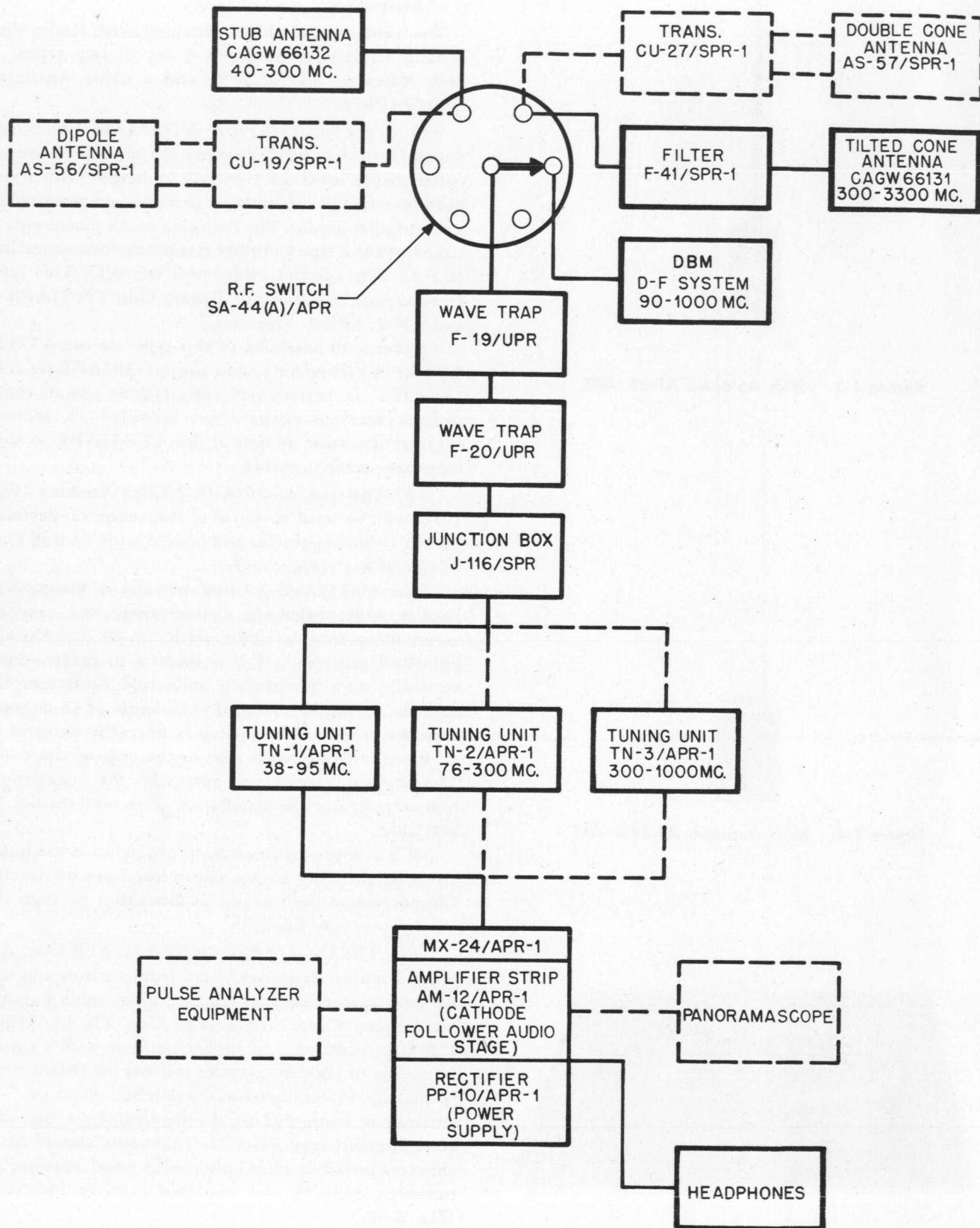
Figure 1-6. Radio Receiving Equipment AN/SPR-1, Block Diagram.
