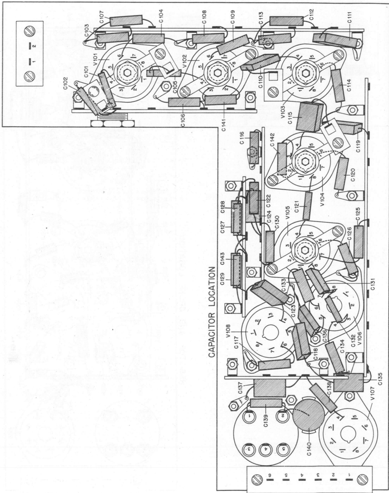
Figure 6-68. Amplifier Strip AM-12/APR-1, Capacitor Location.
