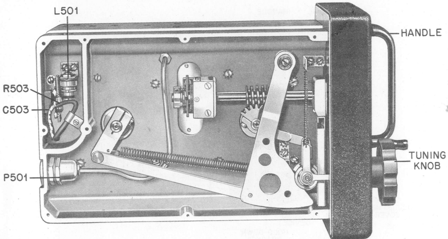
Figure 6-6. Tuning Unit TN-2/APR-1, Left Side View.
