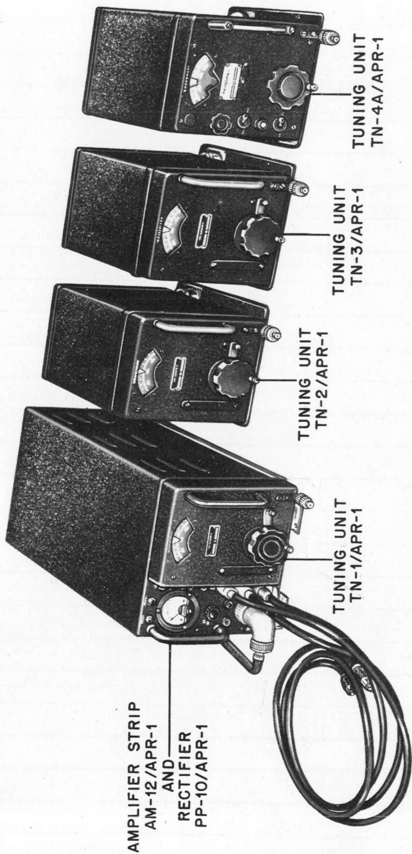
Figure 1-1. Radio Receiving Equipment AN/APR-1 and AN/SPR-1 with Tuning Units.
