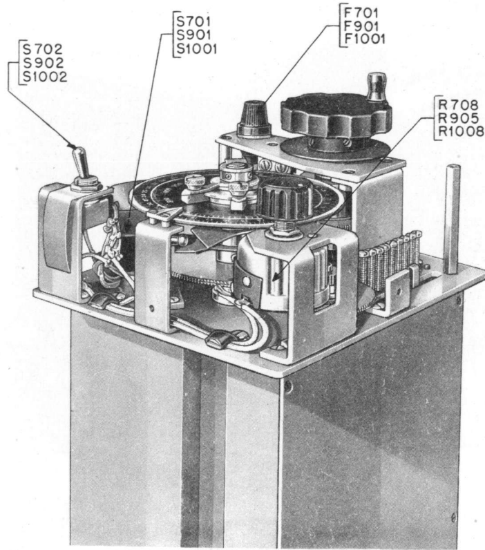
Figure 6-23. Sector Sweep Tuner, Parts Location, Bottom Right Oblique.
