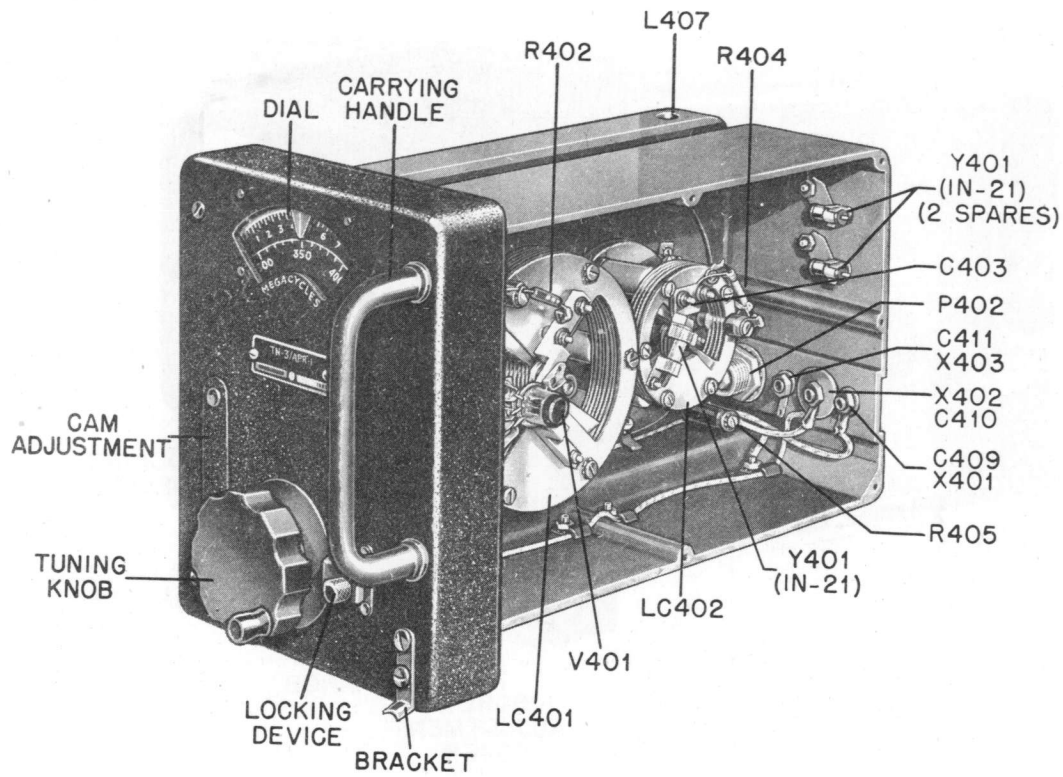
Figure 6-15. Tuning Unit TN-3/APR-1, Right Front Oblique View.
