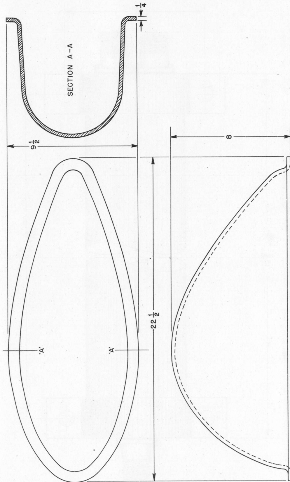
Figure 6-59. Nacelle CW-3/AP, Outline Dimensional.
