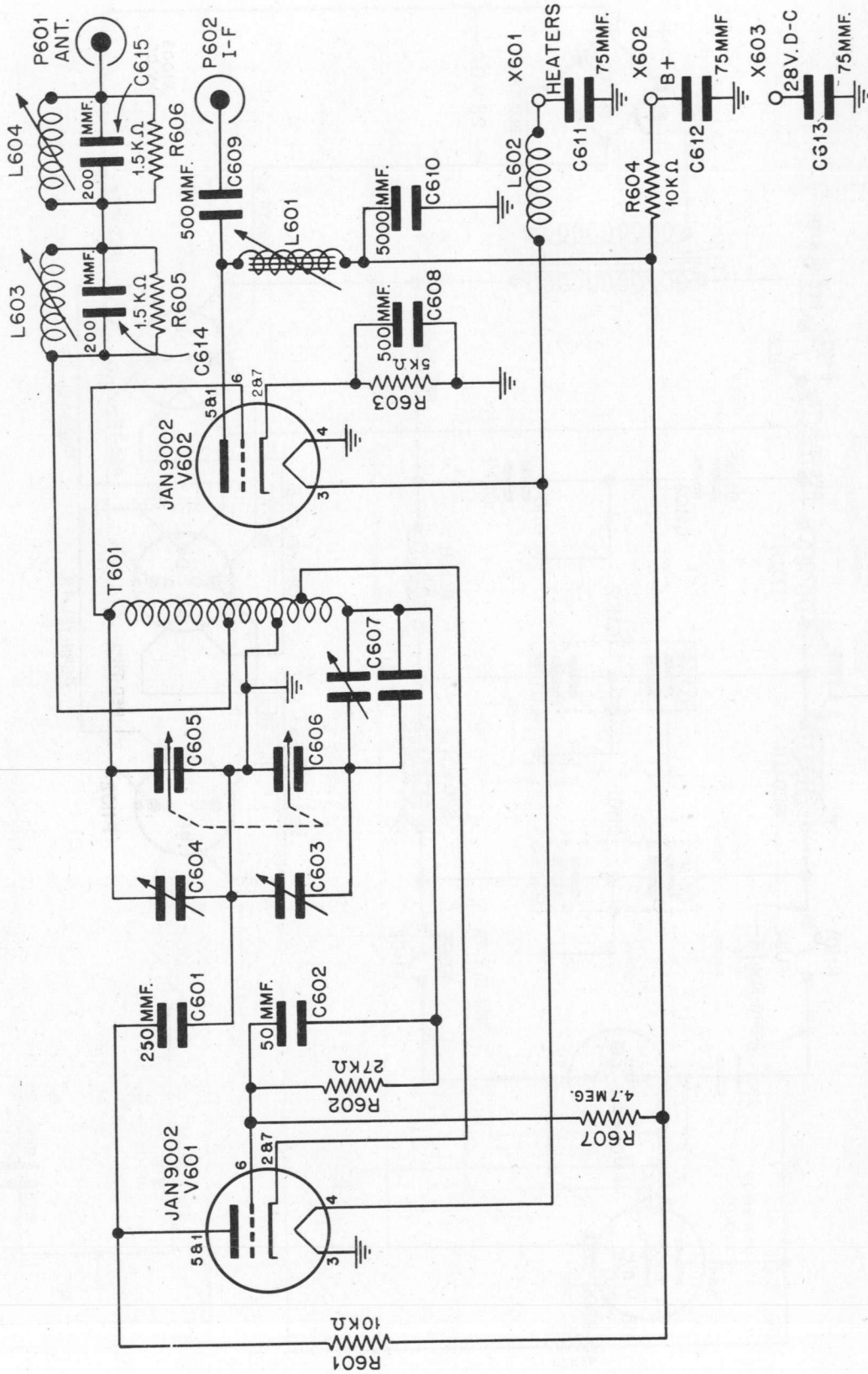
Figure 8-2. Tuning Unit TN-1/APR-1, Schematic Diagram.
