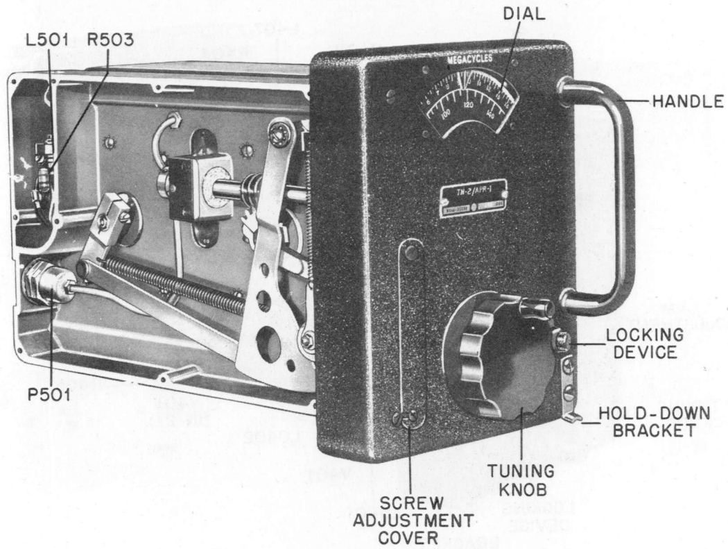
Figure 6-13. Tuning Unit TN-2/APR-1. Left Front Oblique View.
