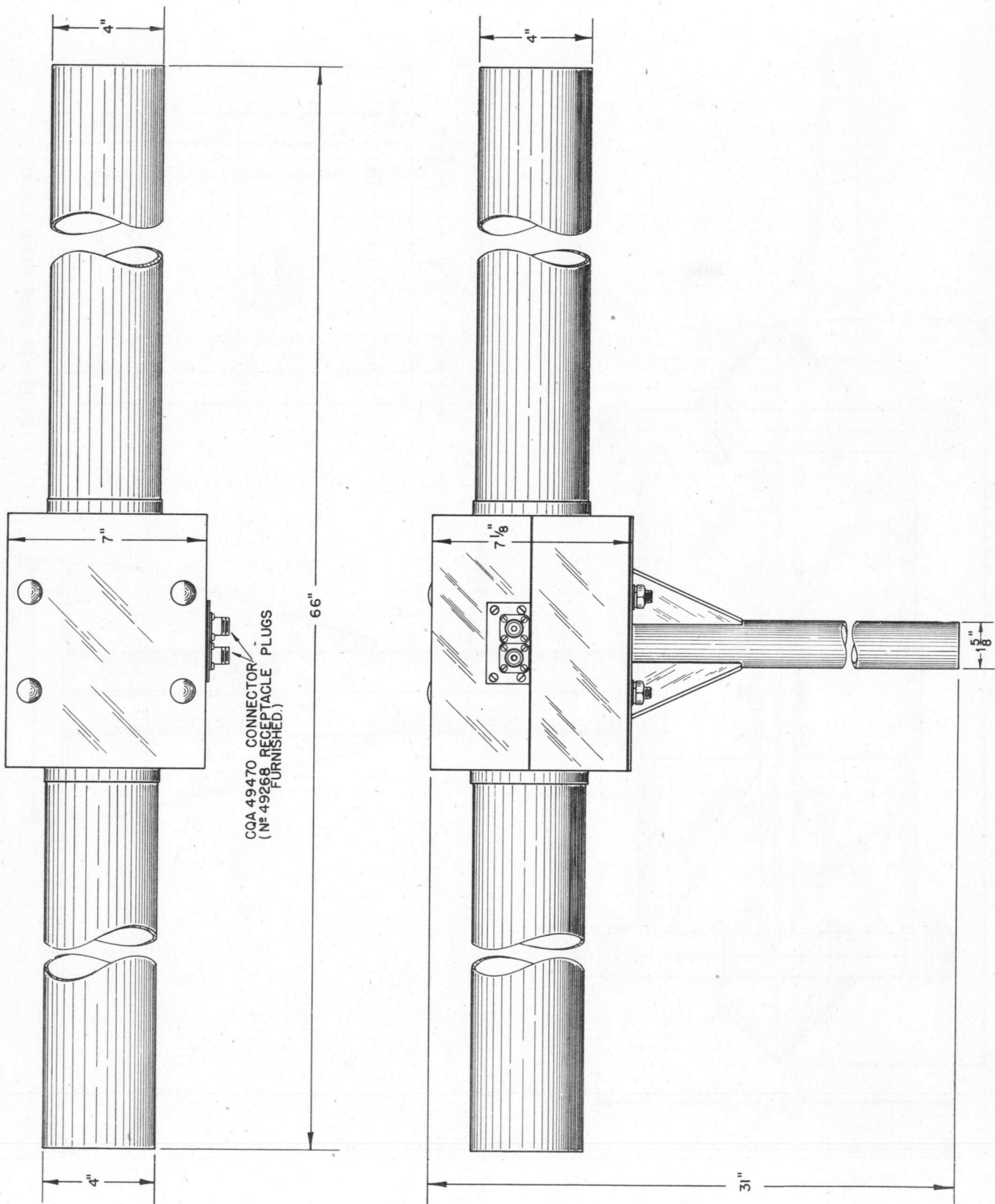
Figure 6-58. Dipole Antenna AS-56/SPR-1, Outline Dimensional.
