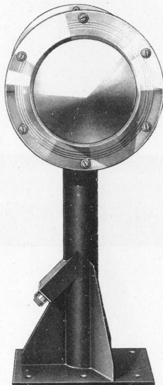
Figure 6-33. Double Cone Antenna AS-57/SPR-1, End View.
