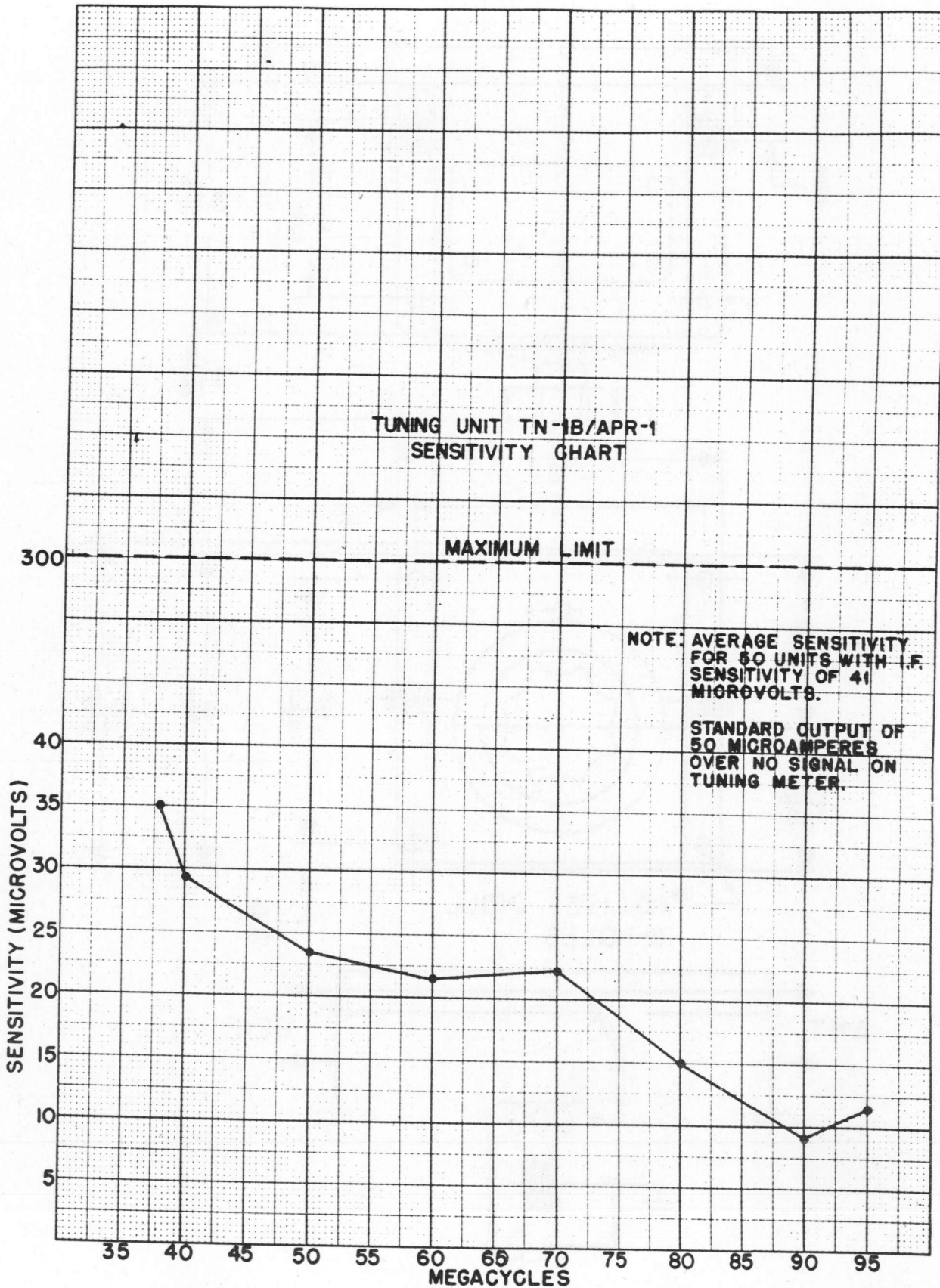
Figure 6-64. Tuning Unit TN-1B/APR-1, Sensitivity Chart.
