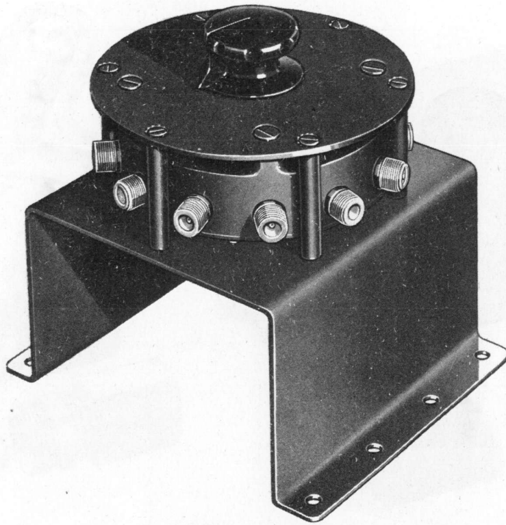
Figure 6-38. Radio Frequency Switch SA-14/SPR-1.
