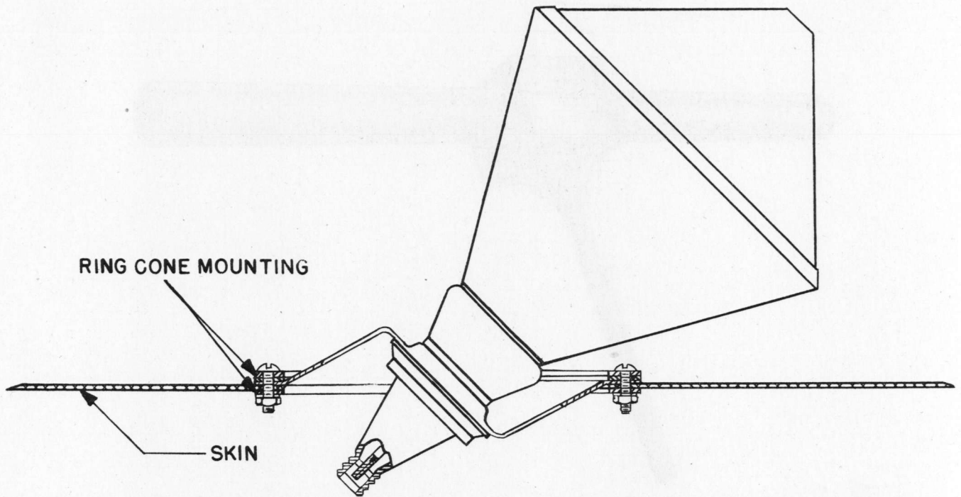
Figure 6-28. Antenna AS-124/APR Outline.
