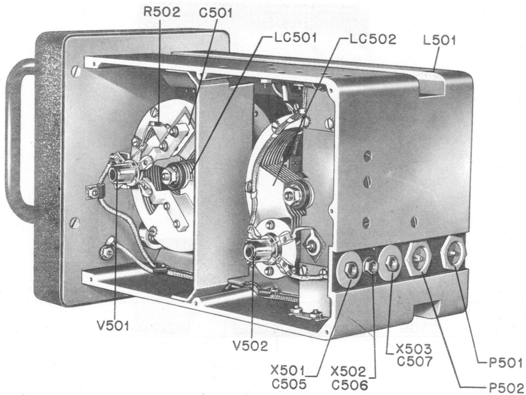
Figure 6-12. Tuning Unit TN-2/APR-1, Rear Left Oblique View.
