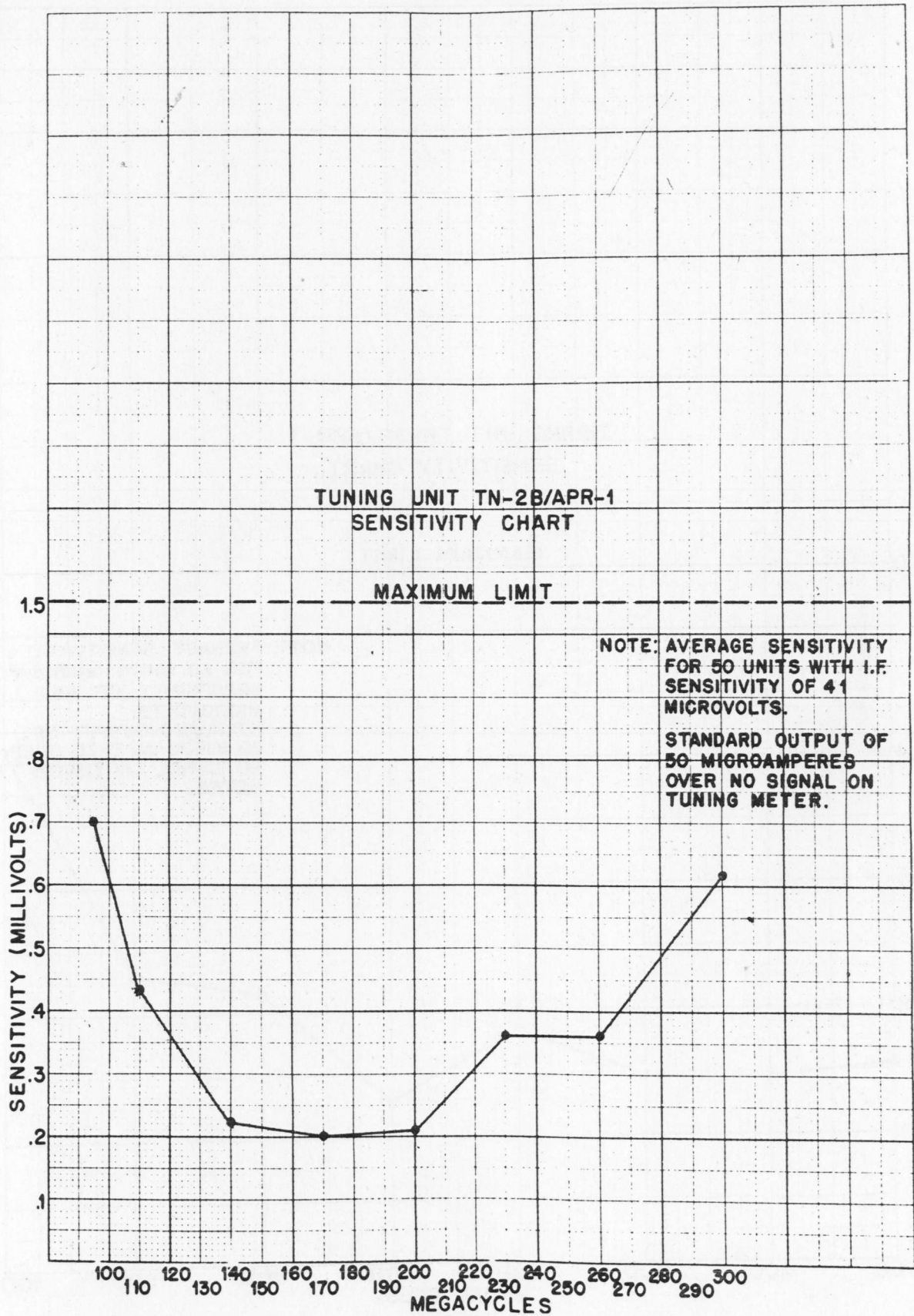
Figure 6-65. Tuning Unit TN-2B/APR-1 Sensitivity Chart.
