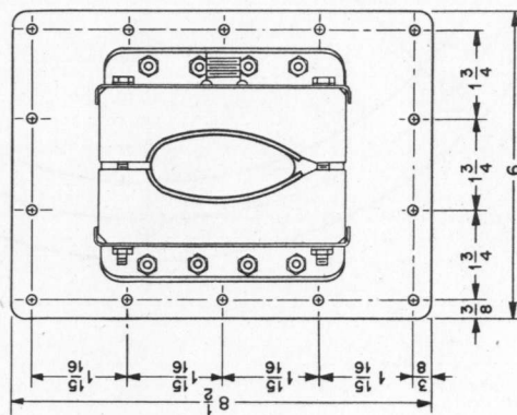
Figure 6-55. Antenna AT-37/APT, Outline Dimensional.
