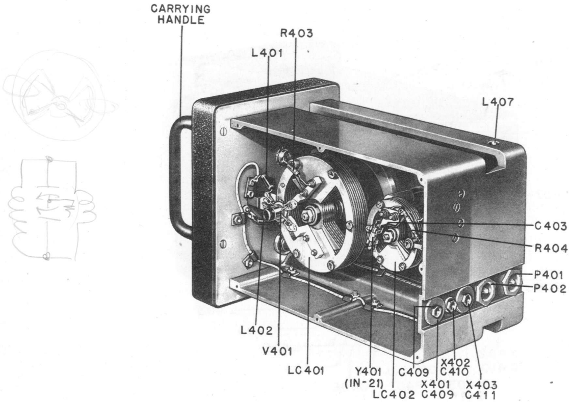
Figure 6-19. Tuning Unit TN-3/APR-1, Rear Right Oblique View.
