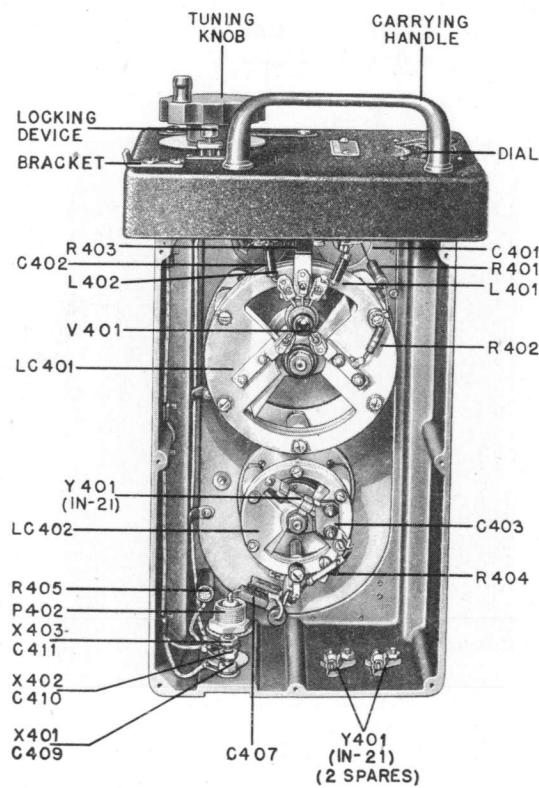
Figure 6-16. Tuning Unit TN-3/APR-1, Right Side View.
