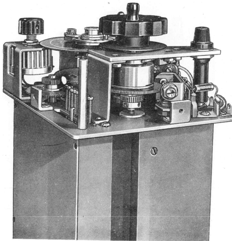
Figure 6-24. Sector Sweep Tuner, Bottom Left Oblique.
