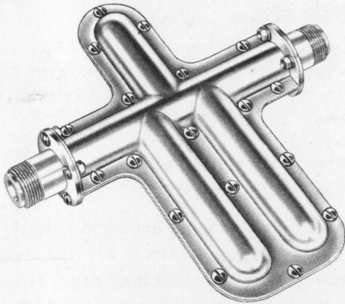
Figure 1-12. Filter F-41/SPR-1.
