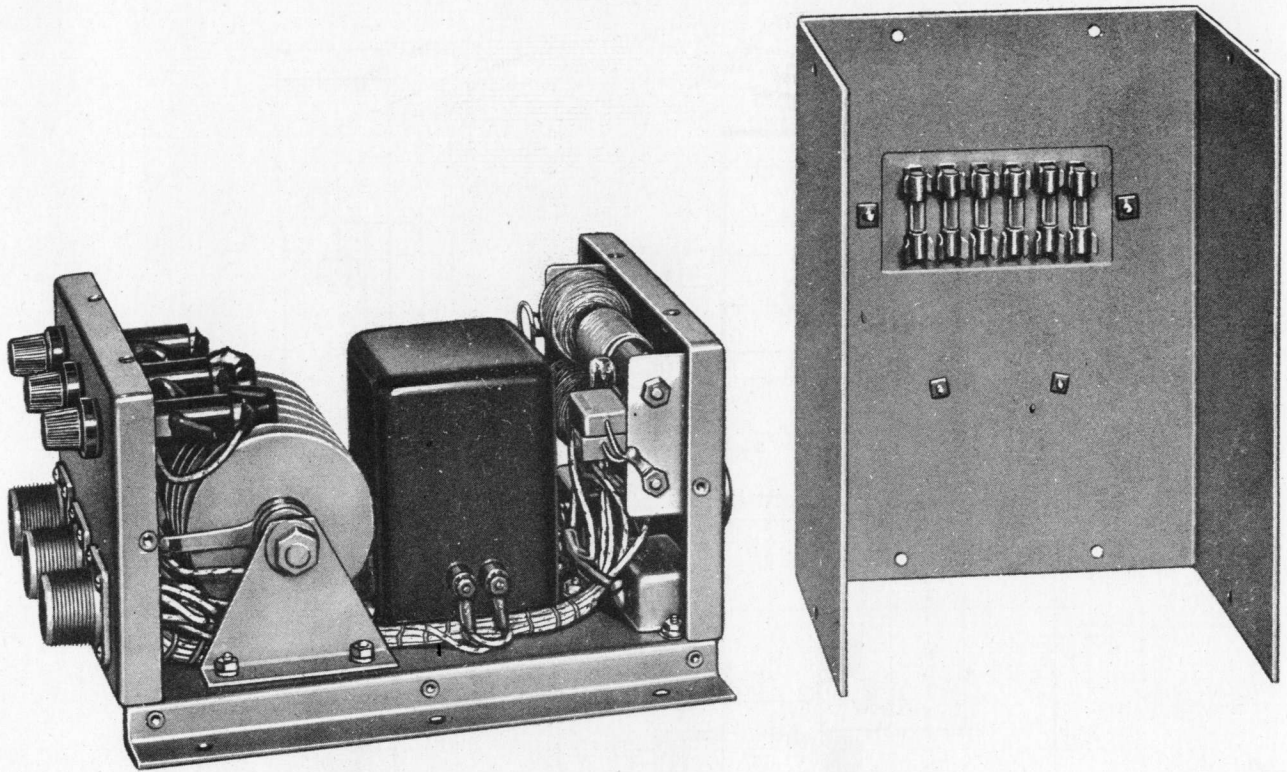
Figure 6-25. Rectifier Filter Unit PP-183/SPR-1, Right Oblique, with Cover.
