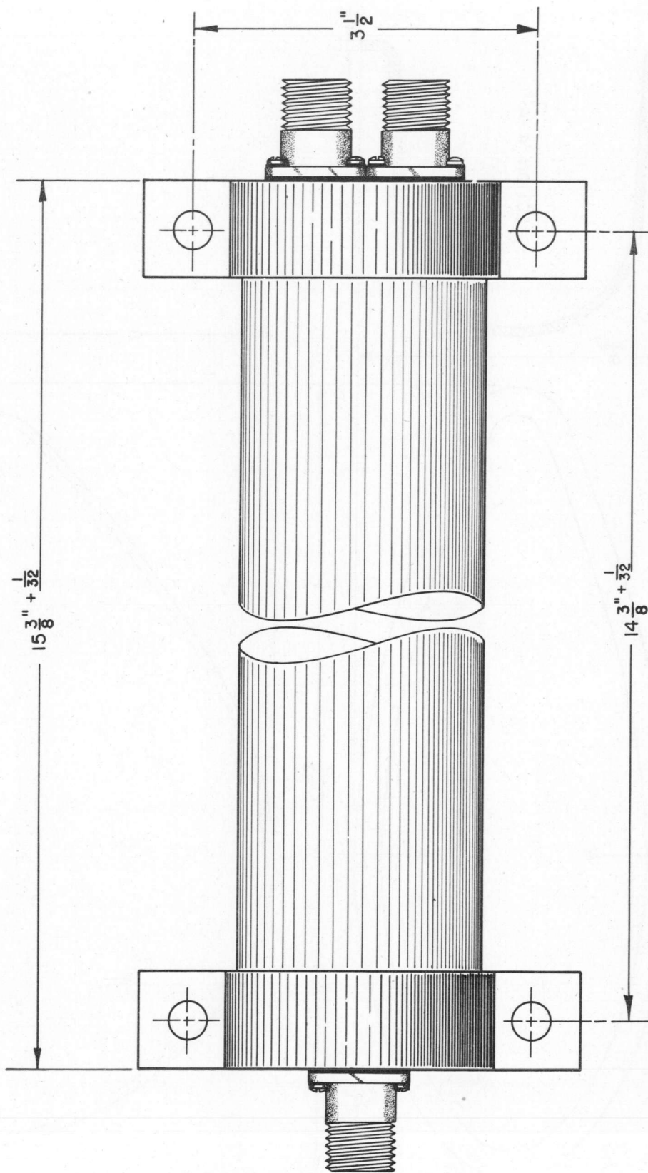
Figure 6-60. Impedance Matching Transformer CU-27/SPR-1, Outline Dimensional.
