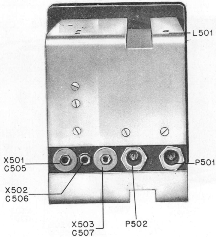
Figure 6-10. Tuning Unit TN-2/APR-1, Rear View.
