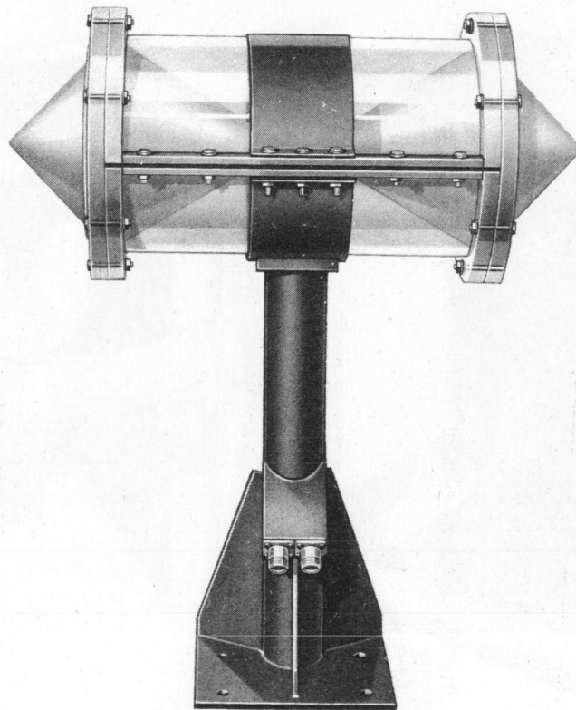
Figure 6-31. Double Cone Antenna AS-57/SPR-1, Side View.
