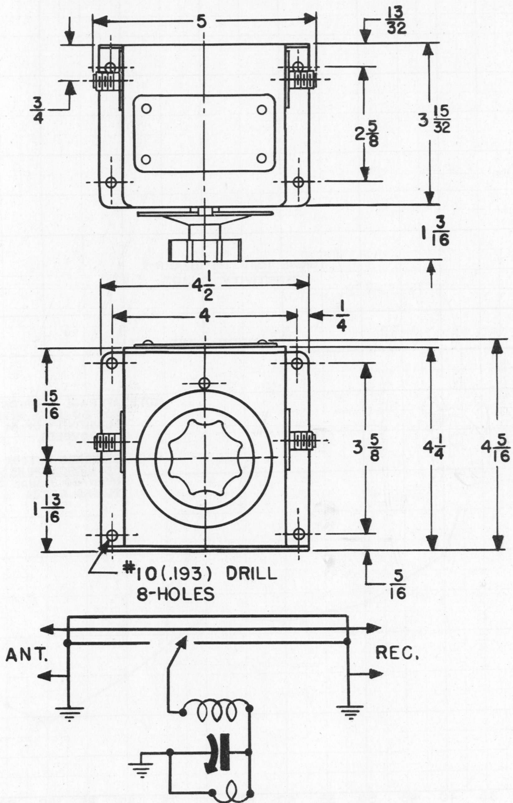
Figure 6-63. Wave Trap F-19/UPR, Outline Dimensional and Schematic.
