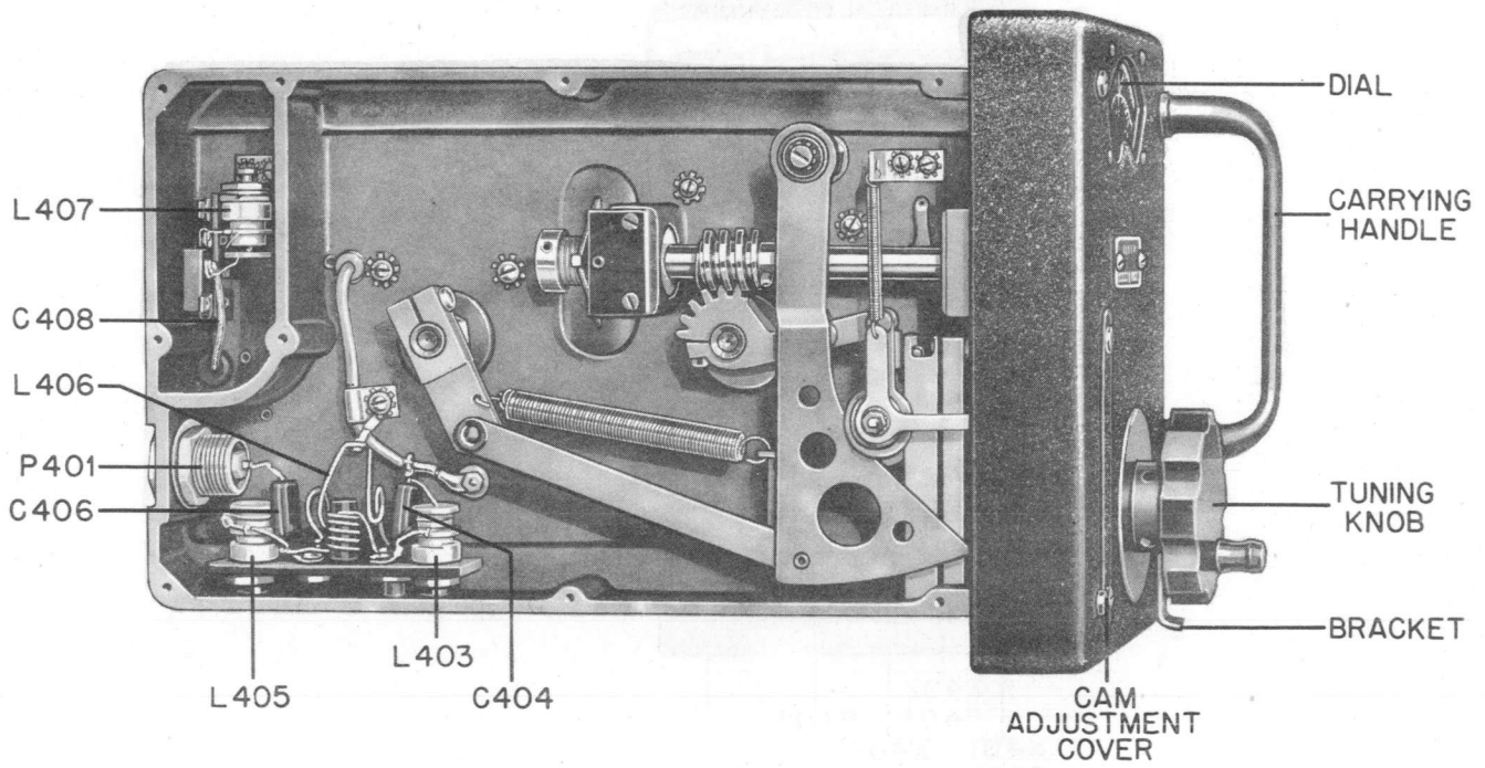
Figure 6-20. Tuning Unit TN-3/APR-1, Left Side View.
