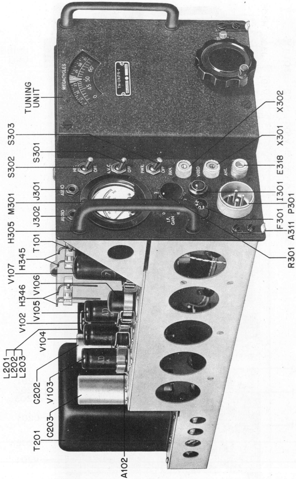
Figure 6-46. Amplifier Strip AM-12/APR-1, Rectifier PP-10/APR-1 and Tuning Unit, Left Front Oblique View.
