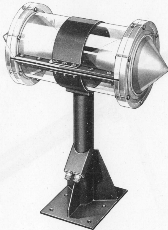
Figure 6-32. Double Cone Antenna AS-57/SPR-1, Oblique View.
