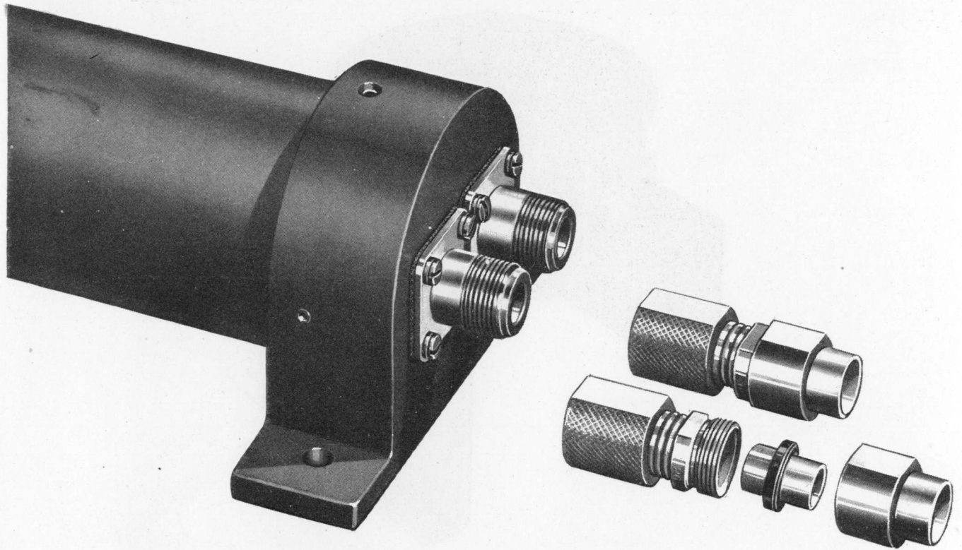
Figure 6-36. Impedance Matching Transformer CU-19/SPR-1 or CU-27/SPR-1, Upper End View.
