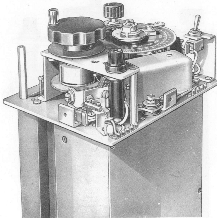
Figure 6-22. Sector Sweep Tuner, Top Left Oblique.
