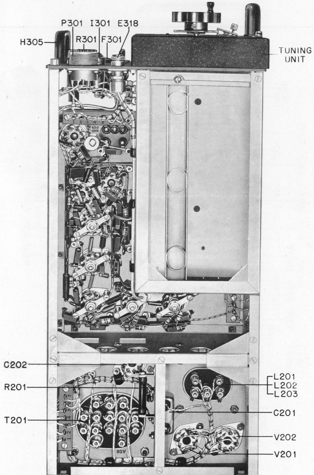
Figure 6-45. Amplifier Strip AM-12/APR-1 and Rectifier PP-10/APR-1, Bottom View.
