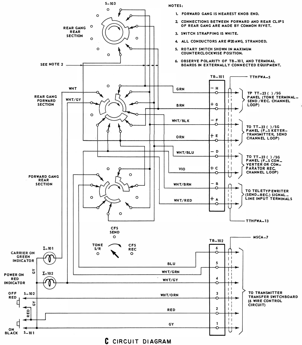
C CIRCUIT DIAGRAM
