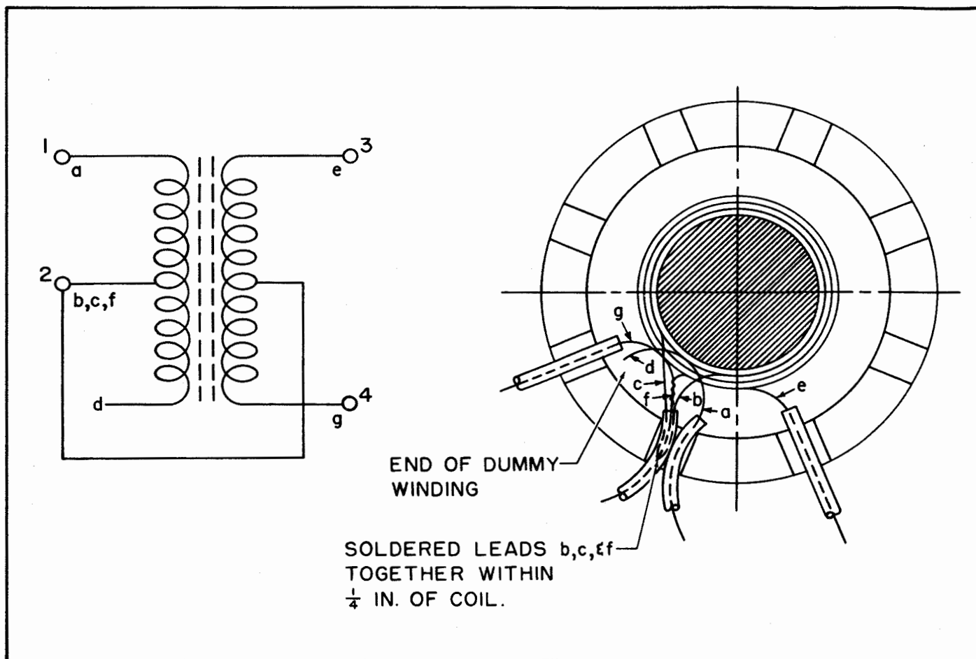
Figure 2-2. Construction of Transformer T-201
