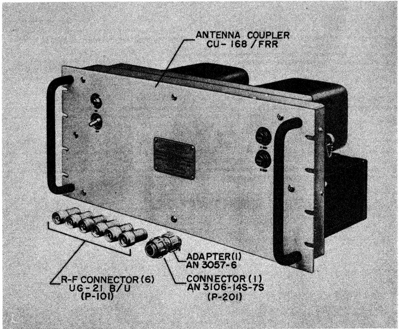
Figure 1-1. Antenna Coupler CU-168/FRR and Accessories
