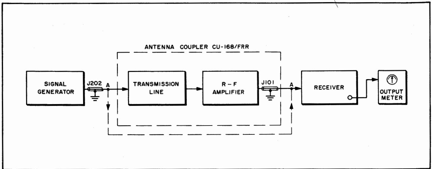
Figure 7-2. Method of Measuring Gain
