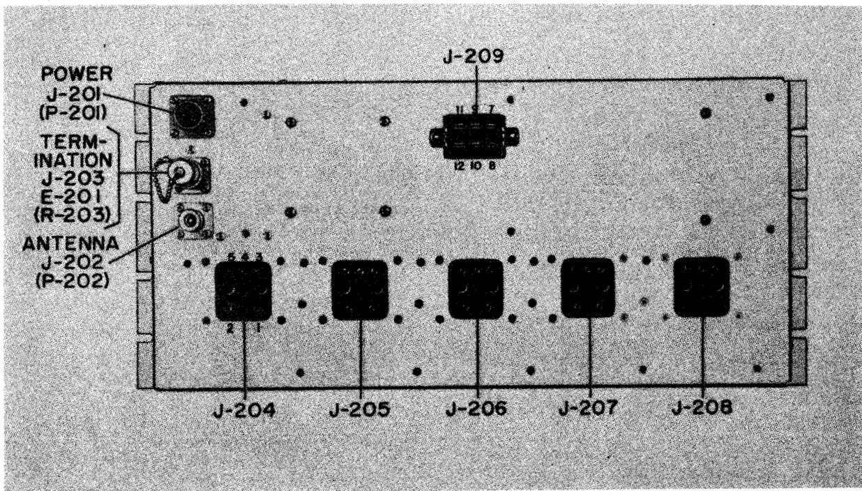
Figure 7-3. Main Chassis, Rear View
