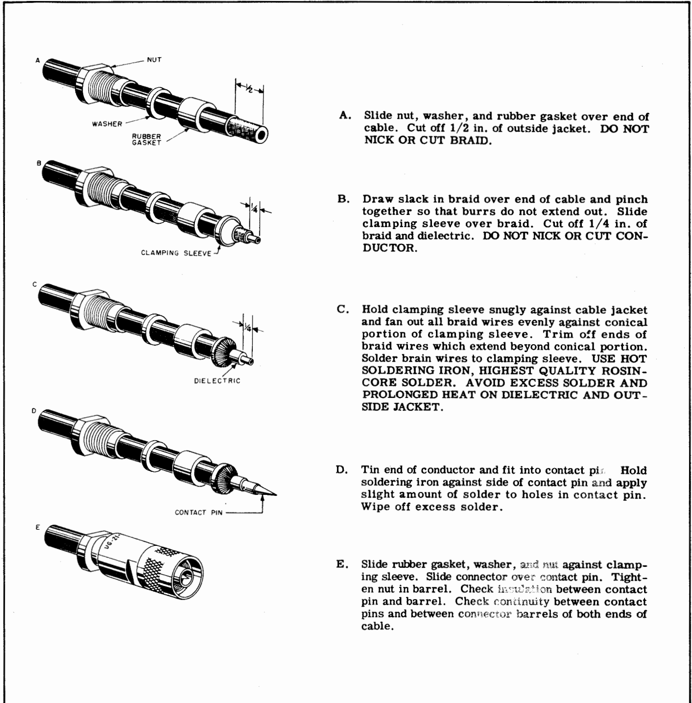
Figure 3-2. Fabrication Instructions for UG-21B/U to RG-11/U
