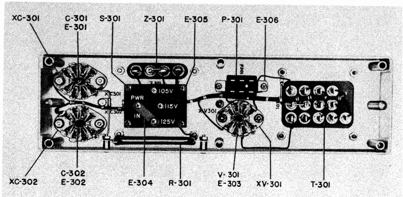
Figure 7-7. Power Supply (PU-301), Front Interior View
