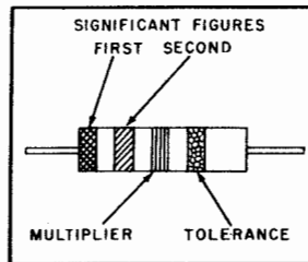
AXIAL TYPE INSULATED
