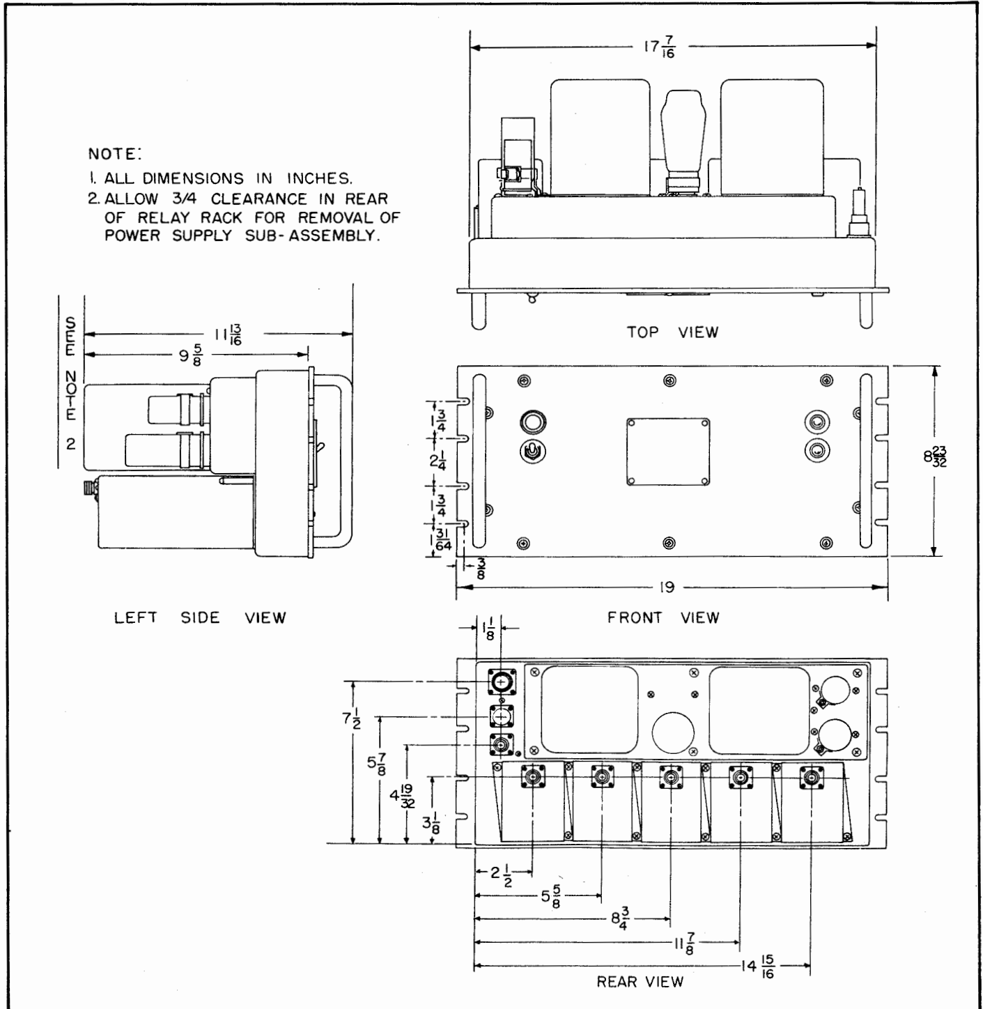
Figure 3-1. Antenna Coupler CU-168/FRR, Dimensional Outline Diagram
