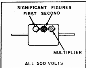
RMA COLOR CODE FOR TUBULAR CERAMIC-DIELECTRIC CAPACITORS
