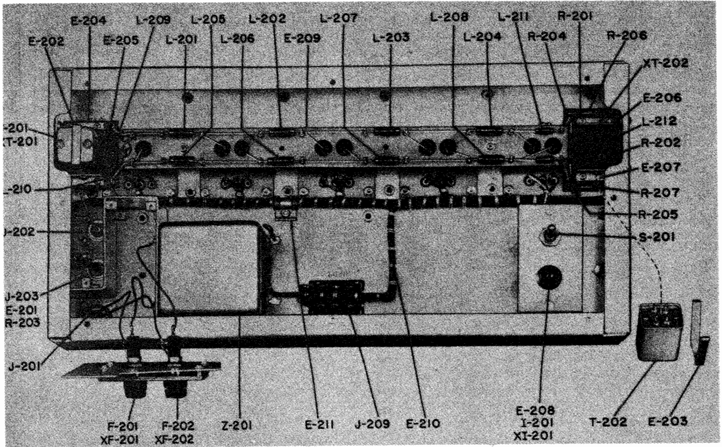
Figure 7-4. Main Chassis, Front Internal View
