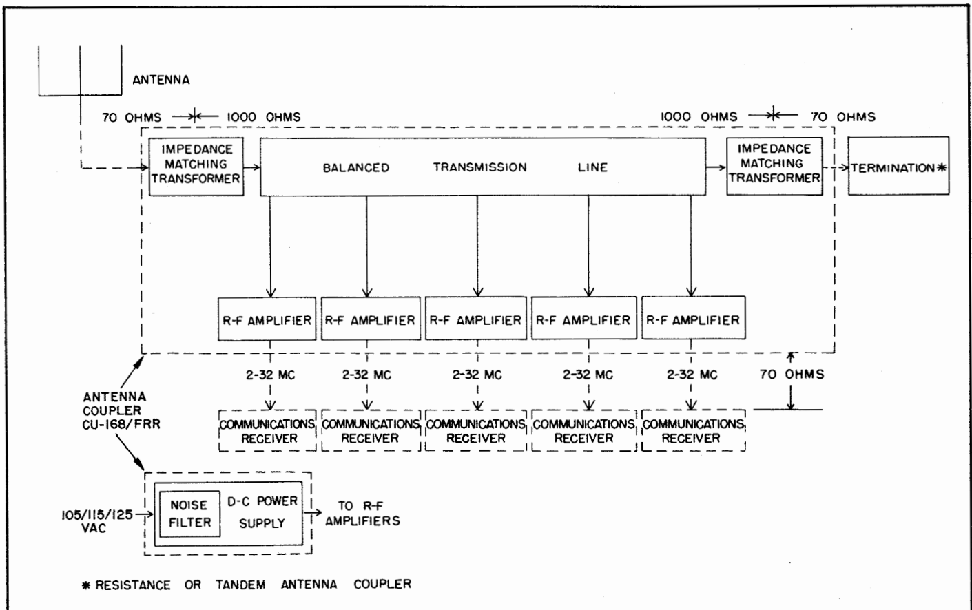
Figure 2-1. Antenna Coupler CU-168/FRR, Block Diagram
