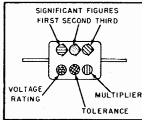
RMA 6-DOT COLOR CODE FOR MICA-DIELECTRIC CAPACITORS
