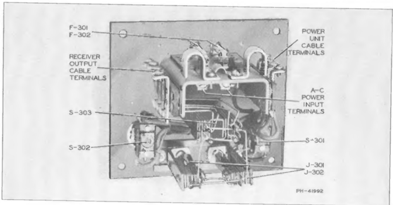
Figure 5—Control Unit CRV-23073 (Rear View of Panel)
