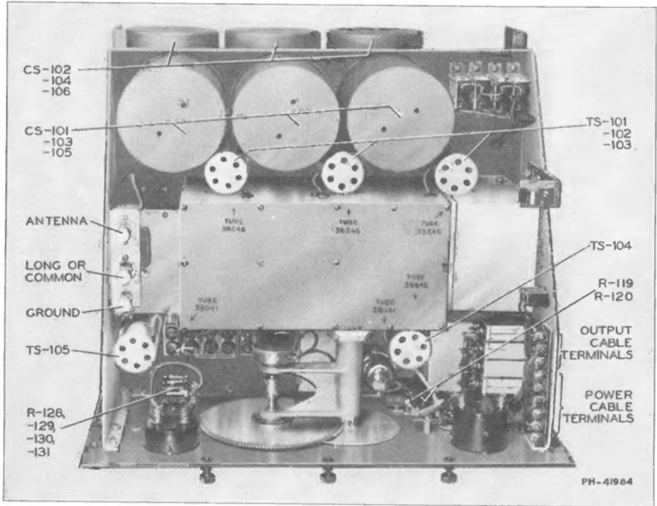
Figure 2—Receiver Unit CRV-46044 (Top View of Chassis)
