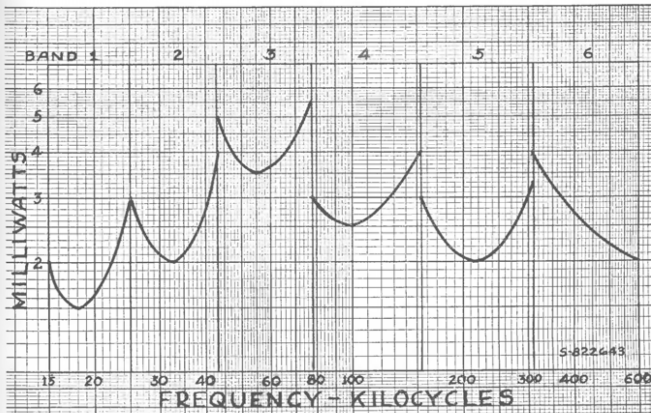
Figure 9—Maximum Noise
