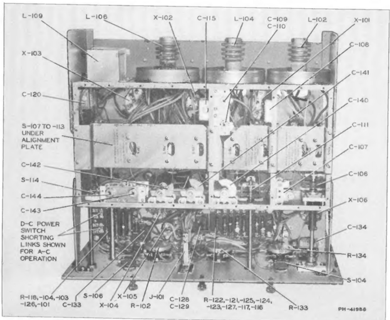
Figure 6—Receiver Unit CRV-46044 (Bottom View of Chassis—Covers Removed)
