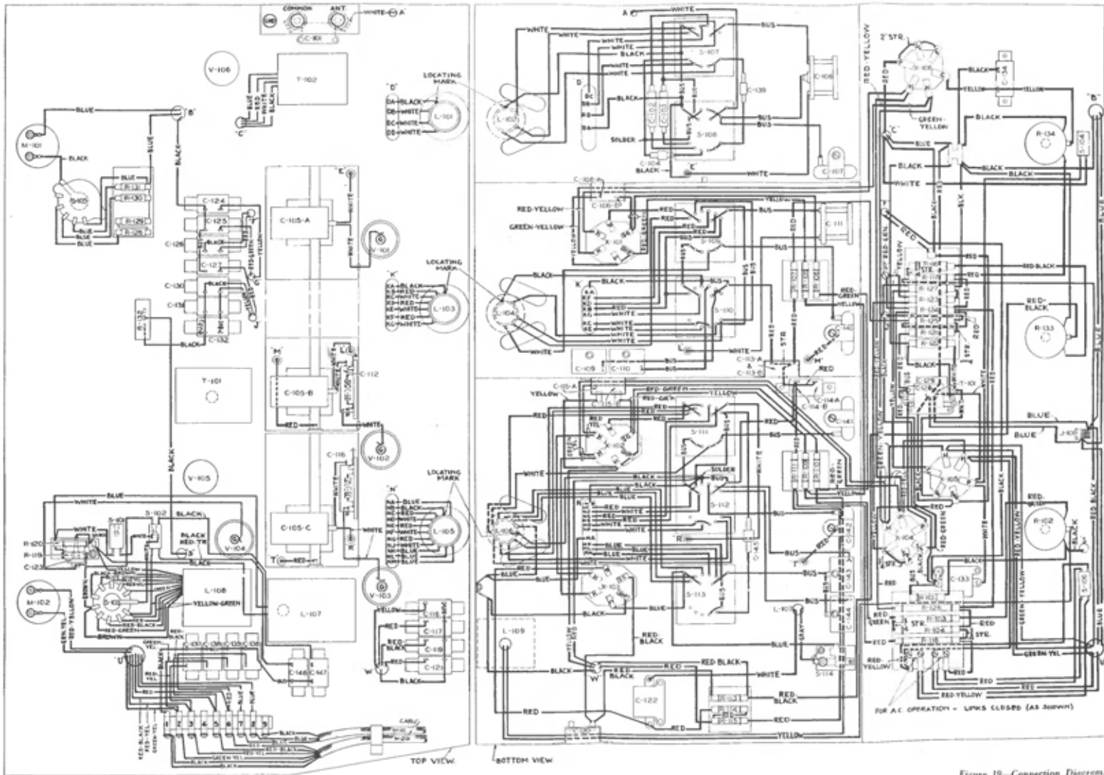
Figure 19—Connection Diagram, Receiver Unit CRV-4604, W-302587
