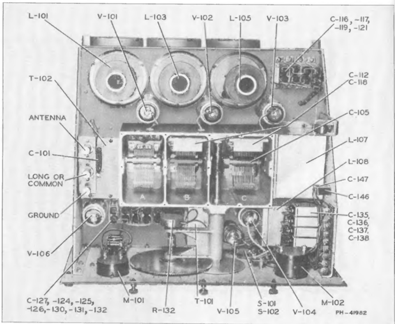
Figure 3—Receiver Unit CRV-4604A (Top View of Chassis—Covers Removed)
