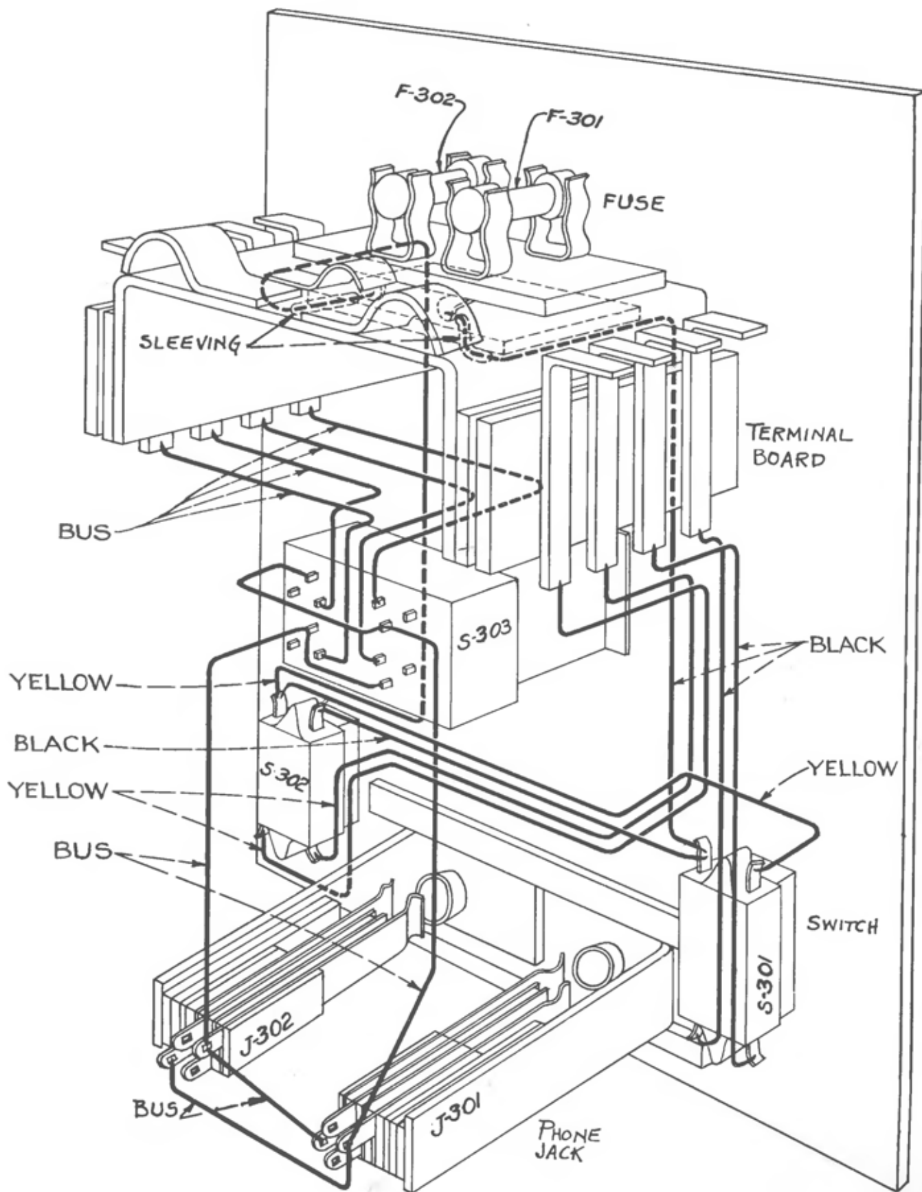
Figure 21—Connection Diagram, Control Unit CRV-23073, P-714101
