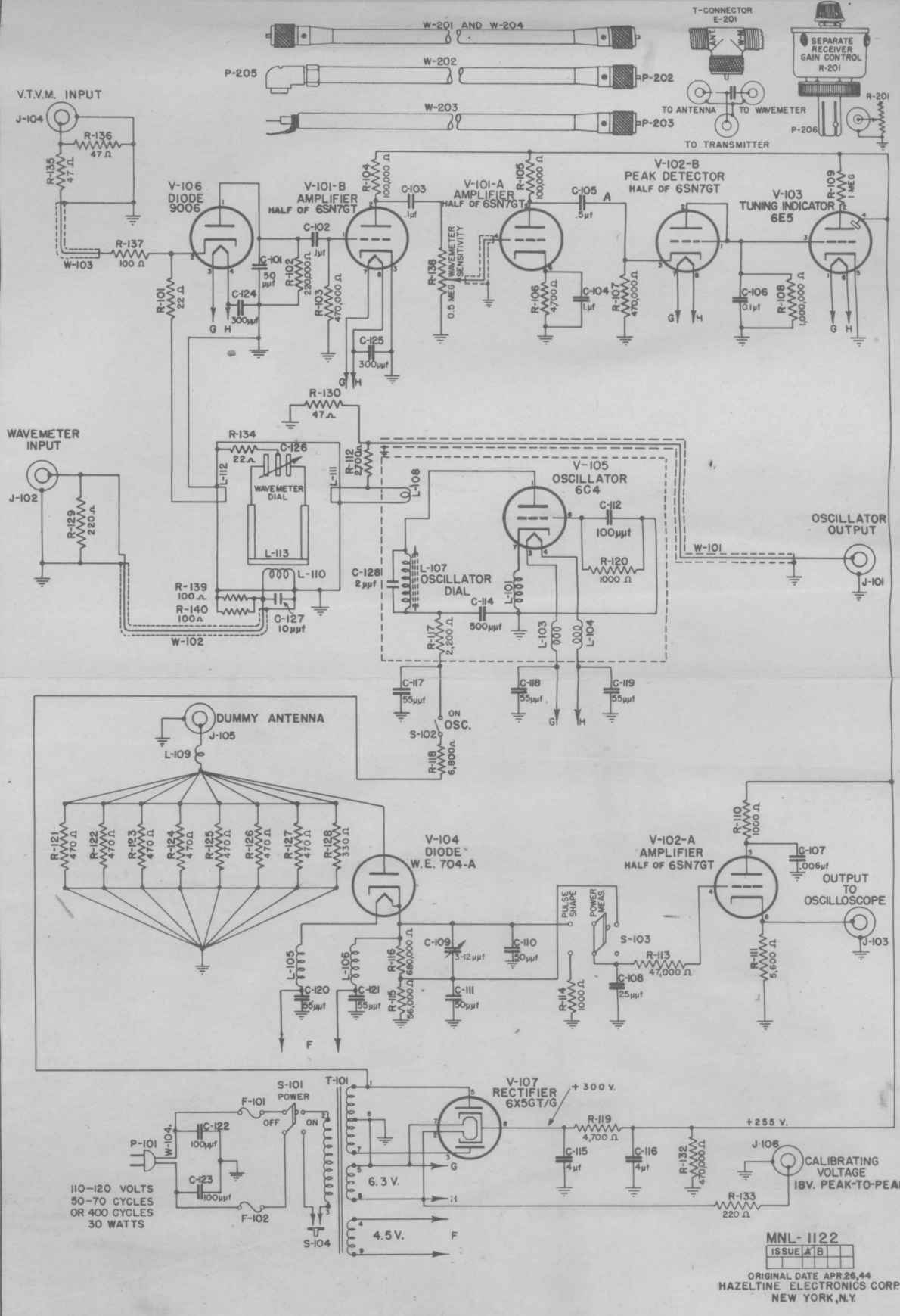
Fig. 9—Schematic Diagram of Model OAP-1 Wavemeter-Oscillator
