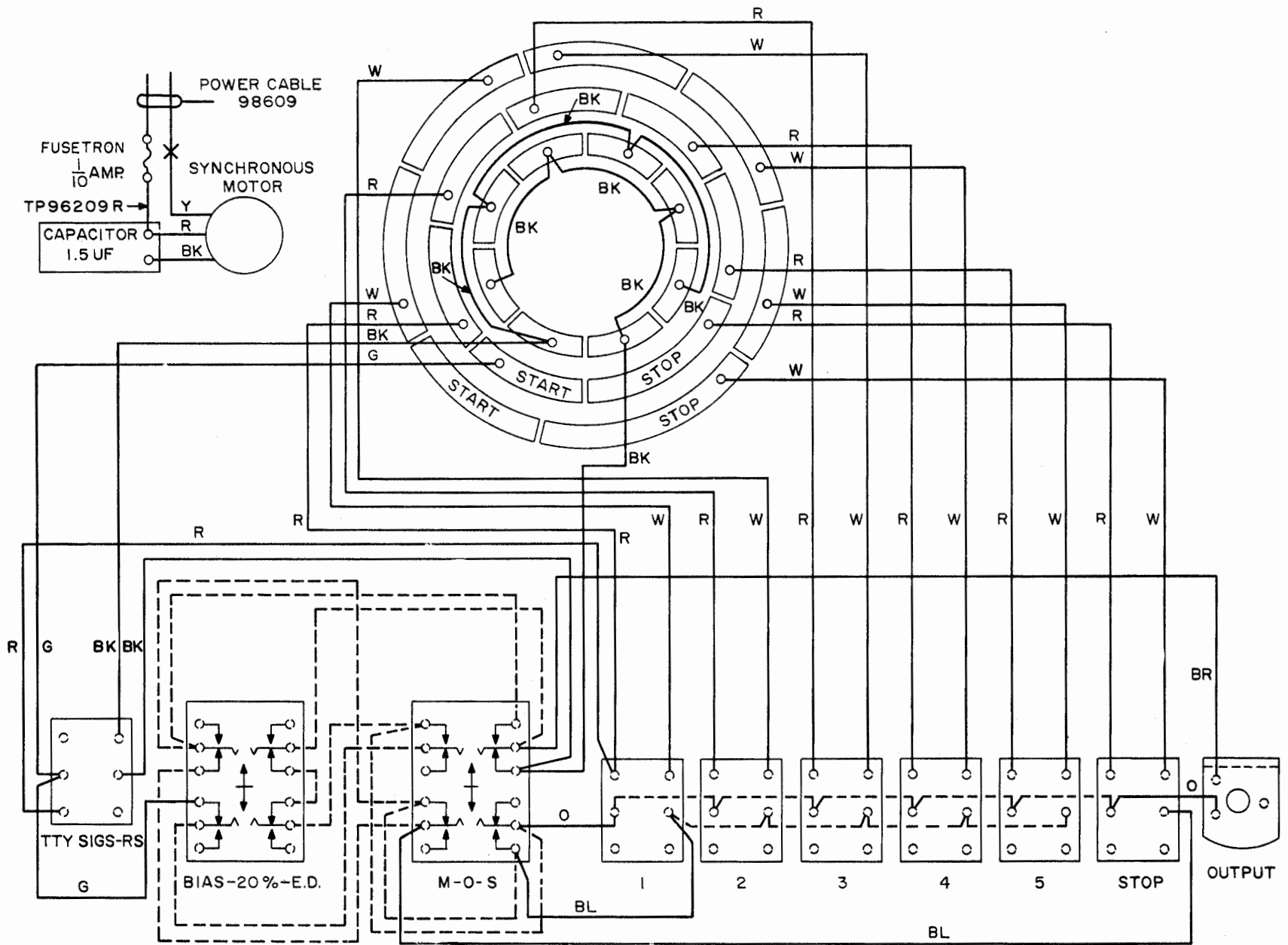
Fig. 3 - 100A Teletypewriter Test Distributor - Wiring Diagram
