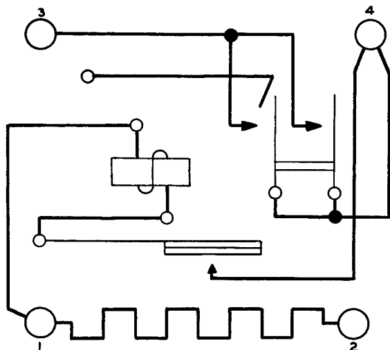
Fig. 2 - Schematic Diagram KS-15623 Relay
