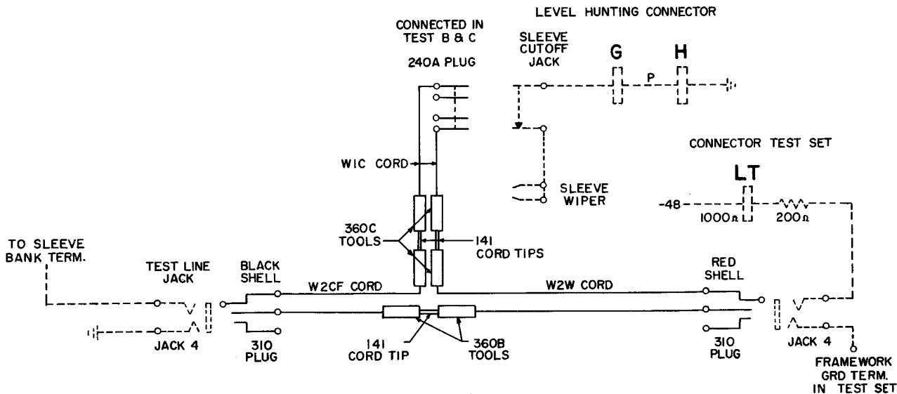
Fig. 1 - Testing Cord
