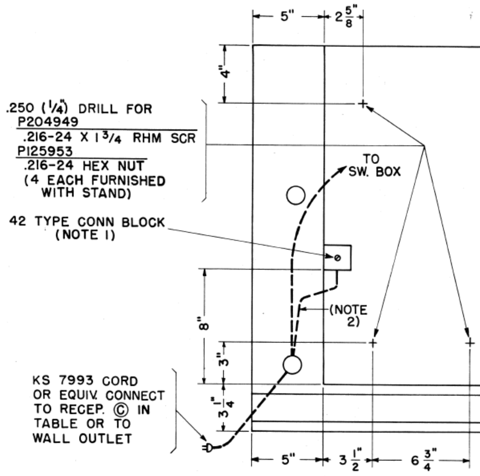
FIG. 3 ED-70225-01 PANEL WITH 128 OR 130 TYPE SUB. S MOUNTED ON ED-91296-01 FLOOR STA
