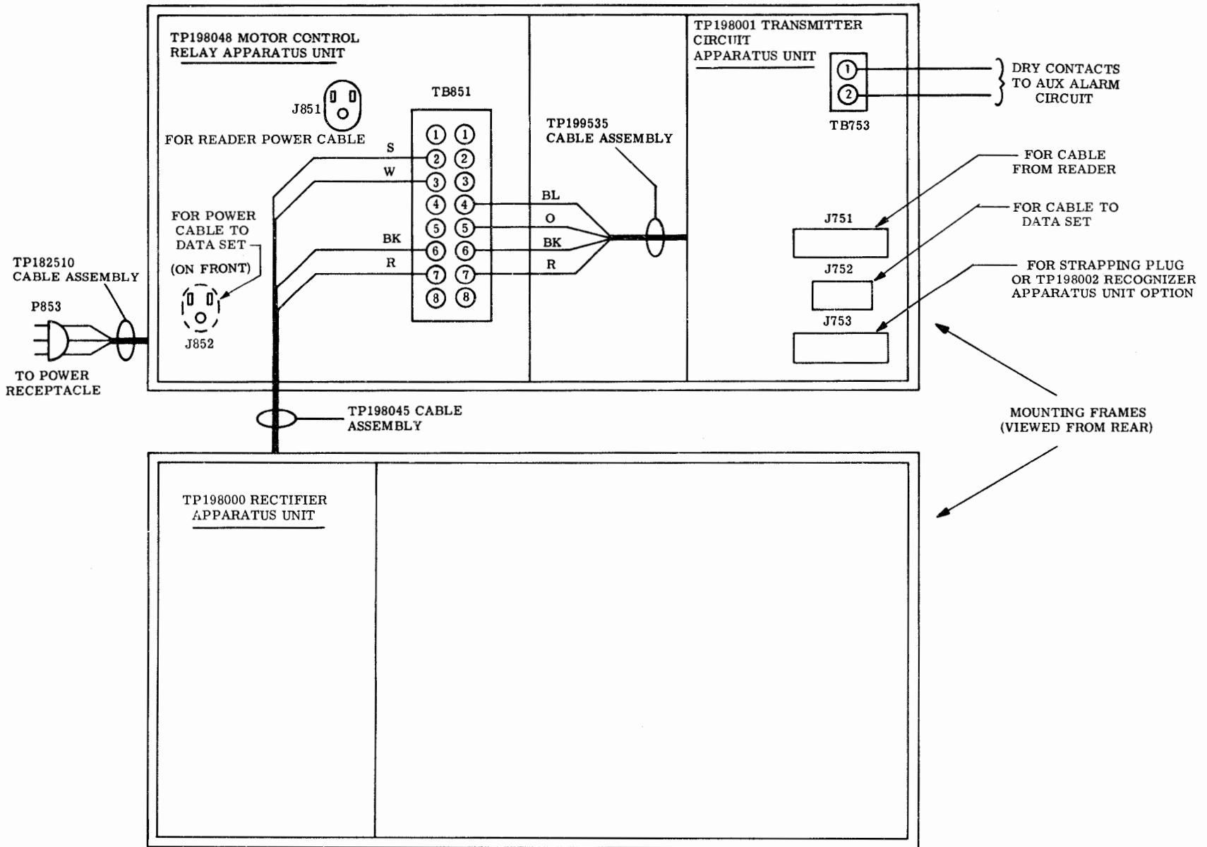
Figure 2 - Tape Senders 5A and 5C Apparatus Unit Connections
