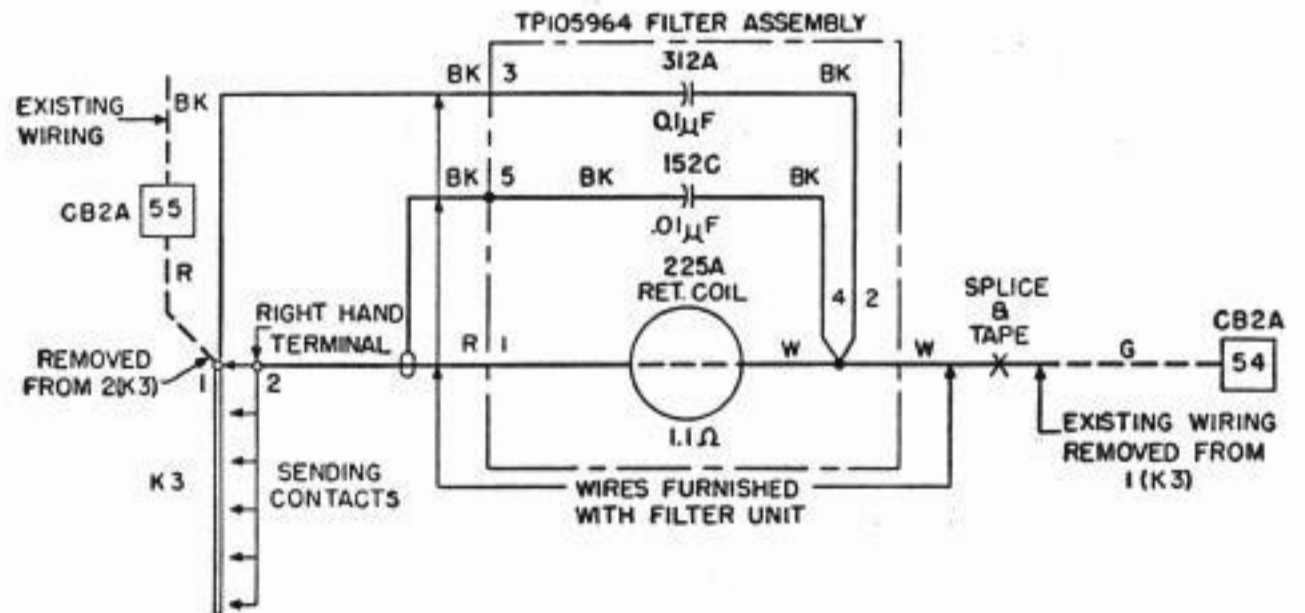
Fig. 2—(Without Line-Test Key) 15D, E, F and G Keyboards
