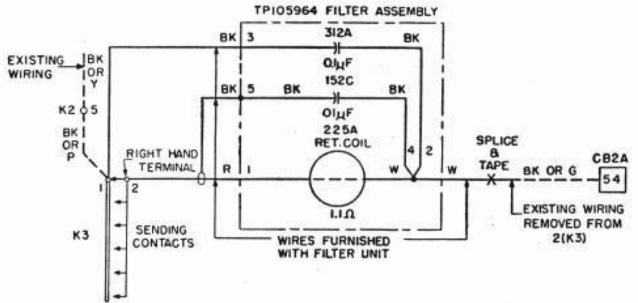
Fig. 1—(With Line-Test Key) 15A, B, and C Keyboards and 15 Type Perforator-Transmitters
