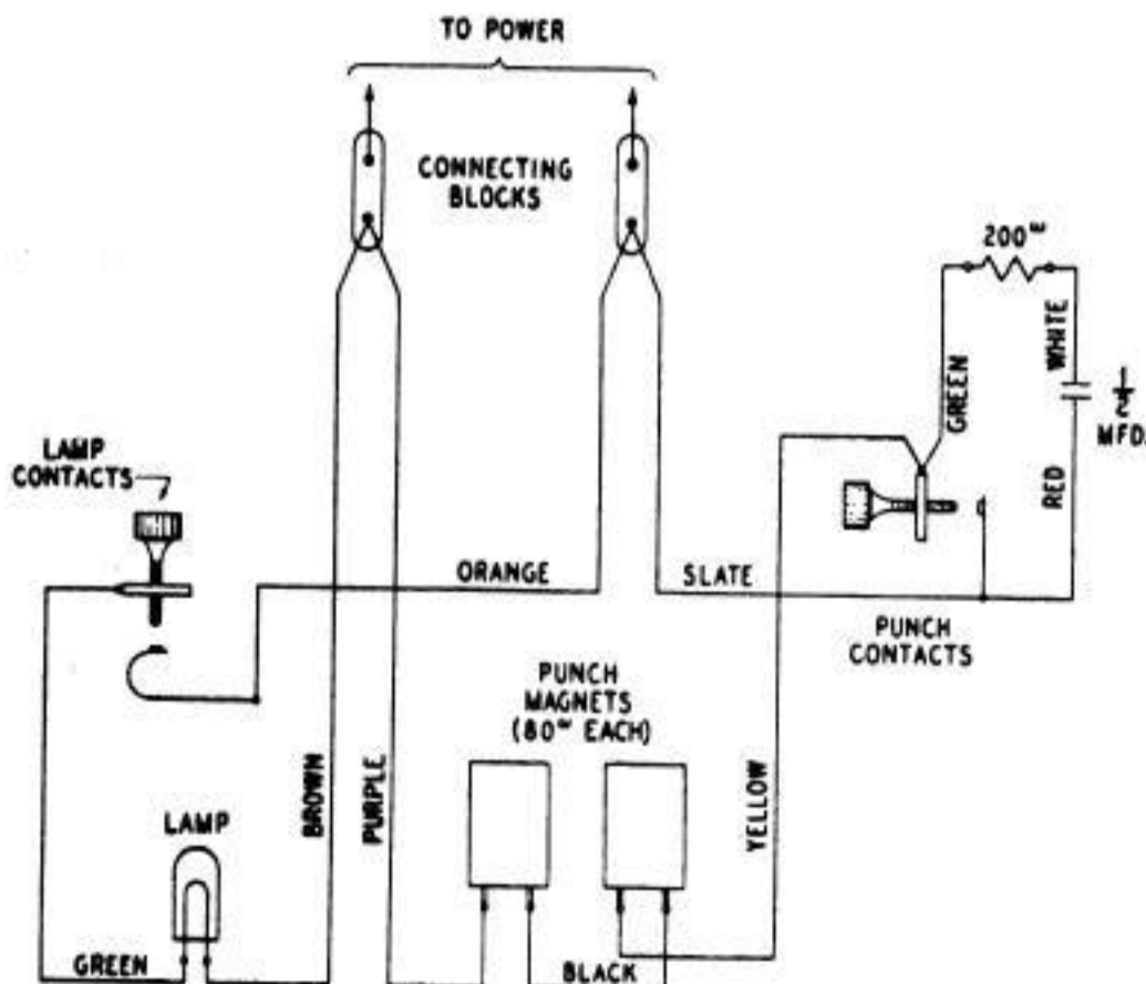
FIG. 1 NO. 14-A AND 13-B TAPE PERFORATOR
