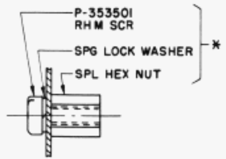
MOUNTING OF SPECIAL NUT ON OUTSIDE OF RIGHT END PANEL SECT. A-A
