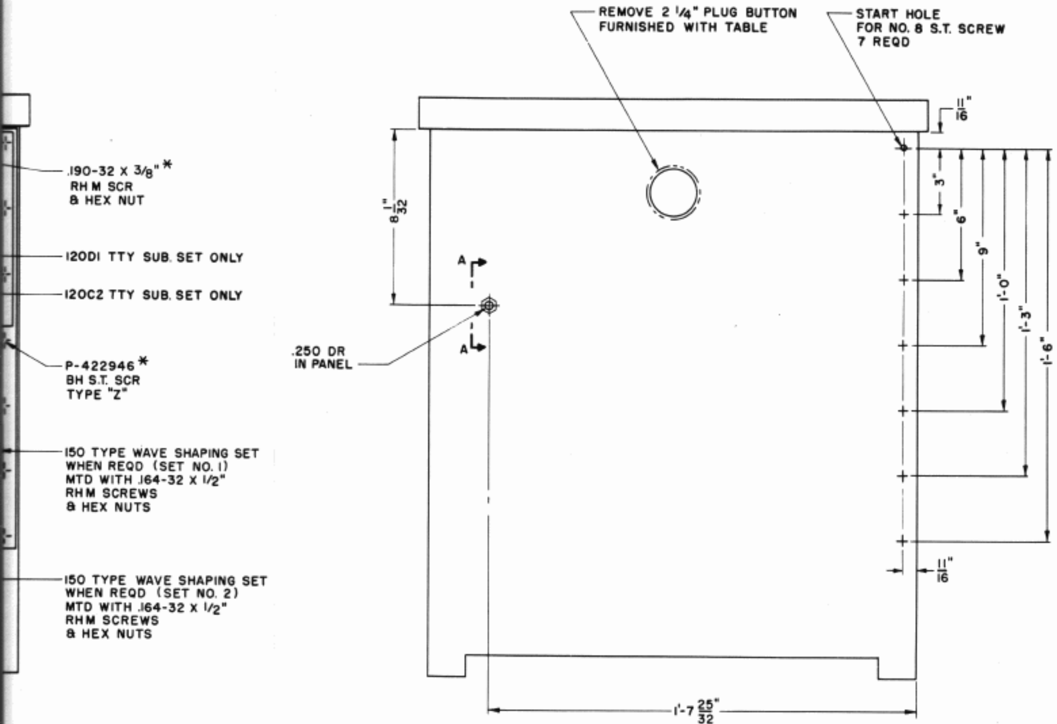
MODIFICATION OF XRT205 OR XRT206 TABLE RIGHT END PANEL ONLY
