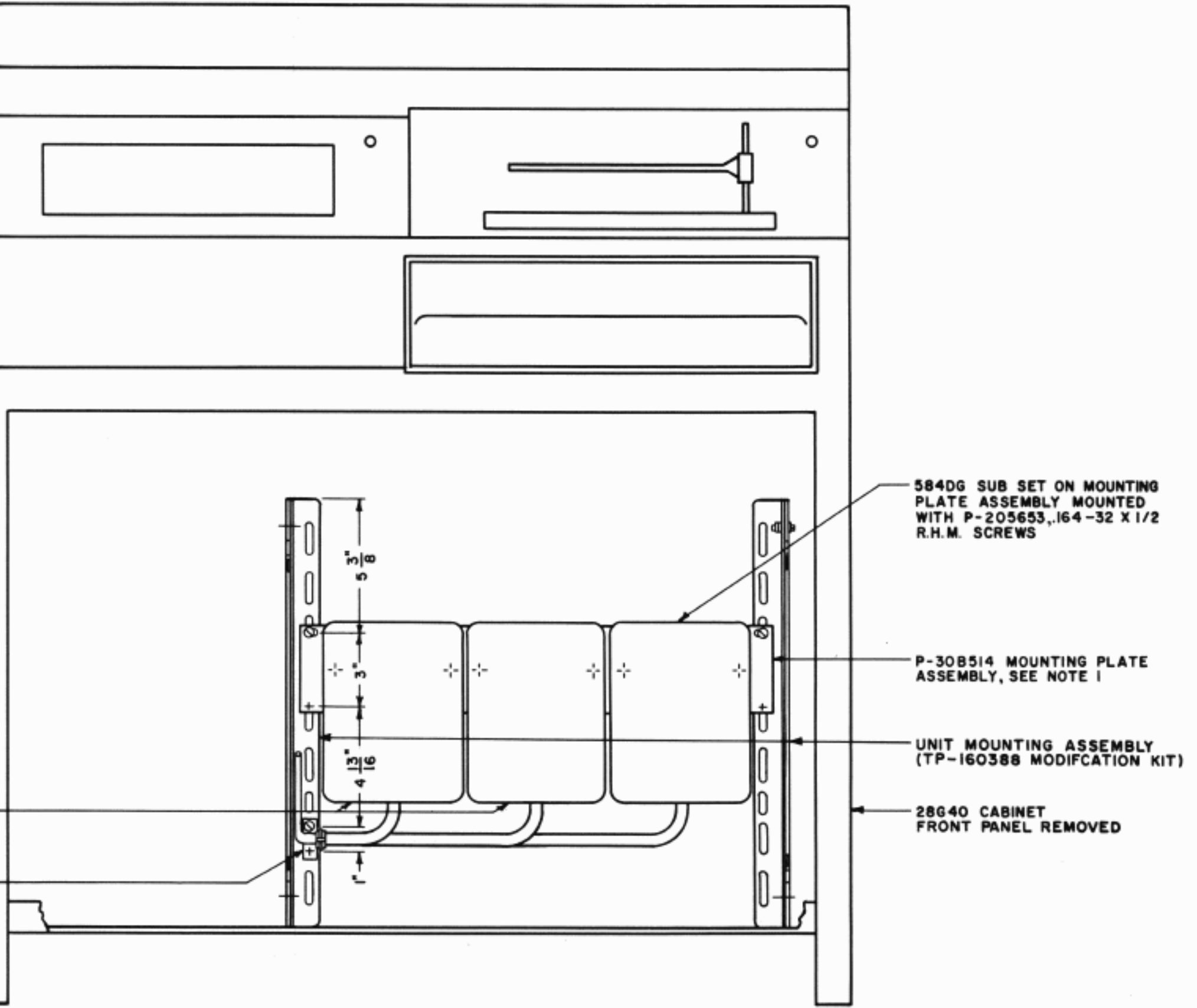
ATTENDED STATION FIG. 2
