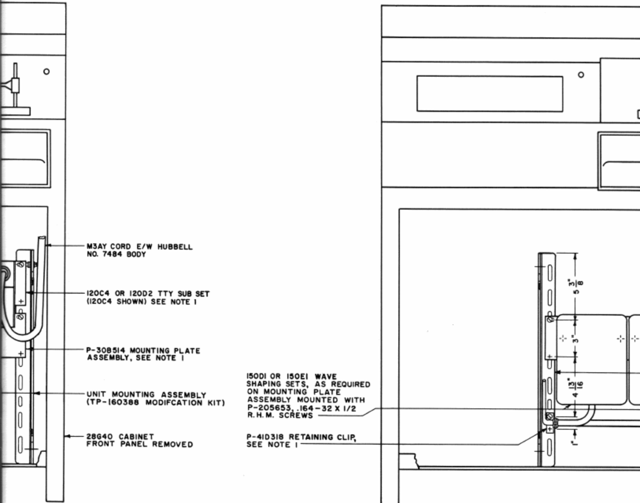
ATTENDED STAT FIG. 2
