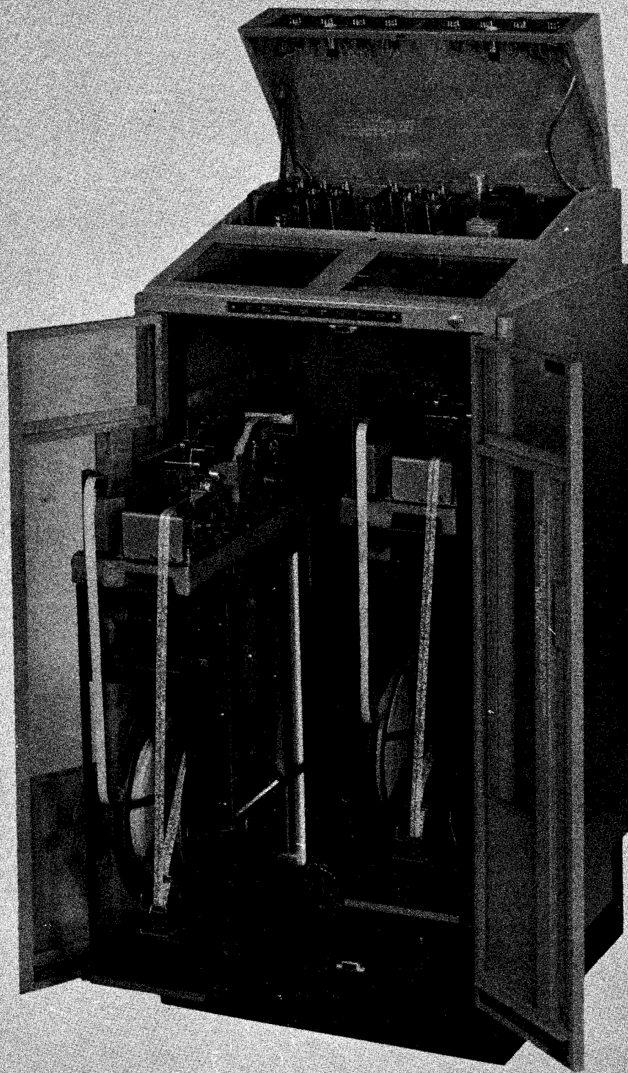
M28 TYPING REPERFORATOR TRANSMITTER DISTRIBUTOR SET
