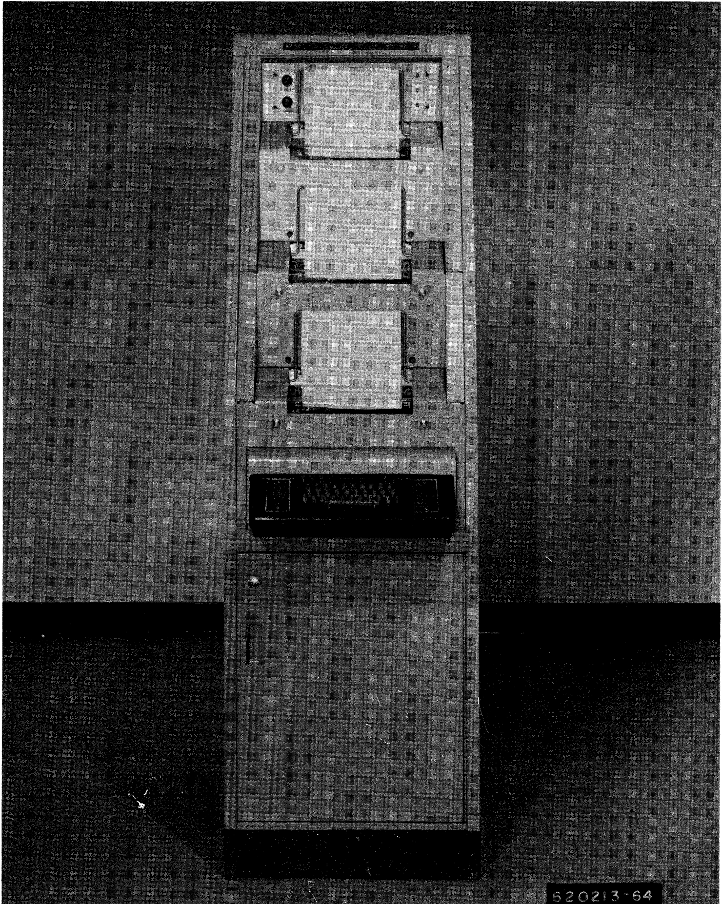
M28 MULTIPLE (STACK) MOUNTED SEND-RECEIVE PAGE PRINTER SET
