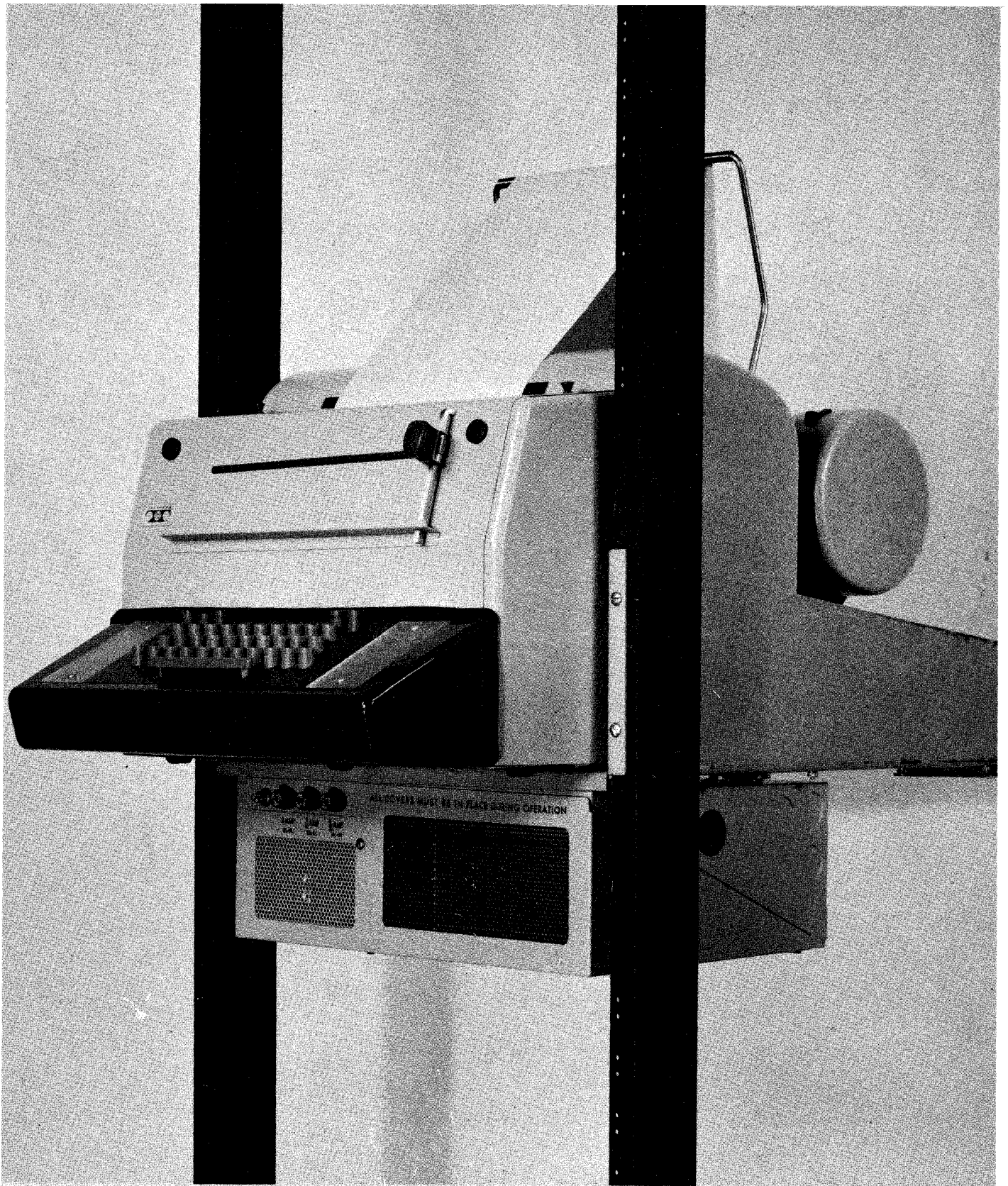
MODEL 28 LOW LEVEL KEYBOARD SEND-RECEIVE SET (RACK MOUNTED)
