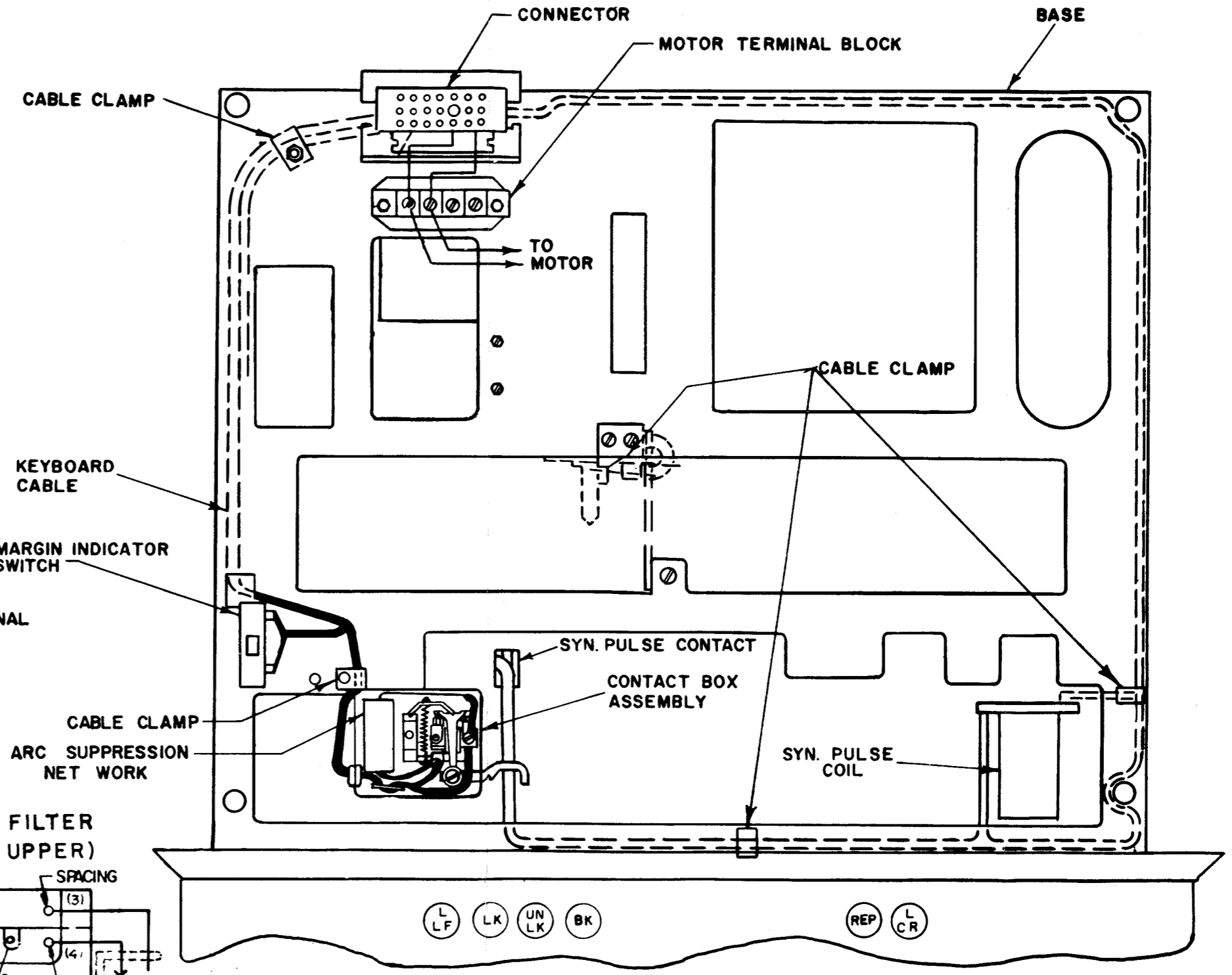
CABLE ROUTING TOP VIEW
