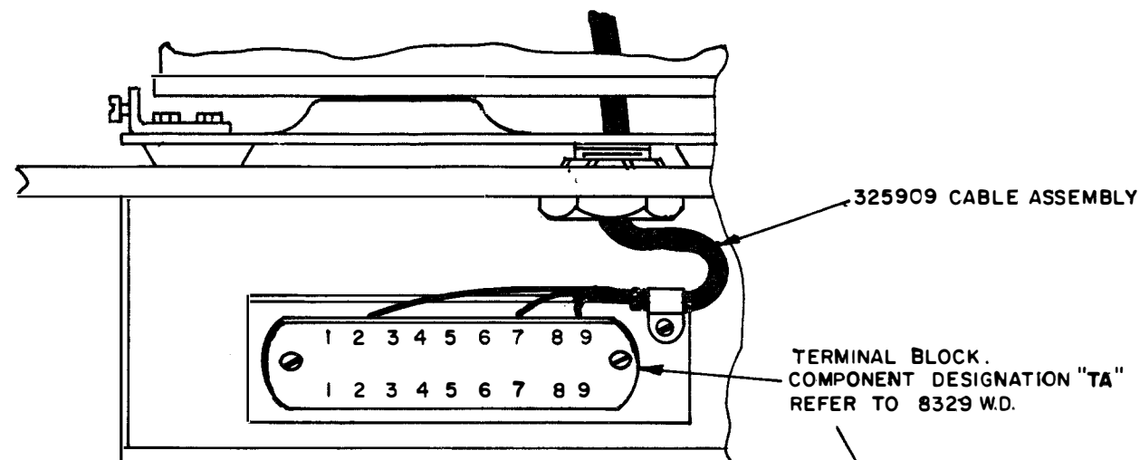
LEFT FRONT VIEW (CABLE ROUTING)
