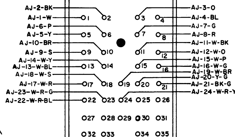
AA TYPING UNIT CONNECTOR ON 325908 CABLE ASSEMBLY
