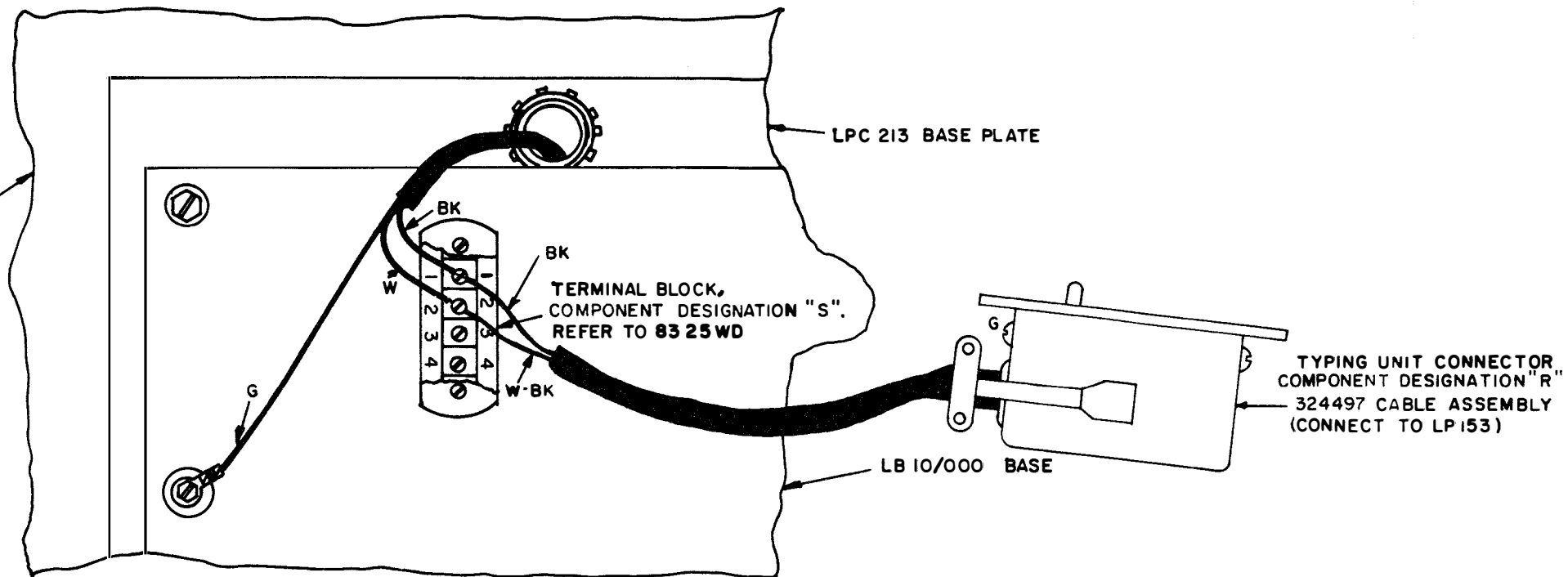
LEFT REAR TOP VIEW (CABLE ROUTING)
