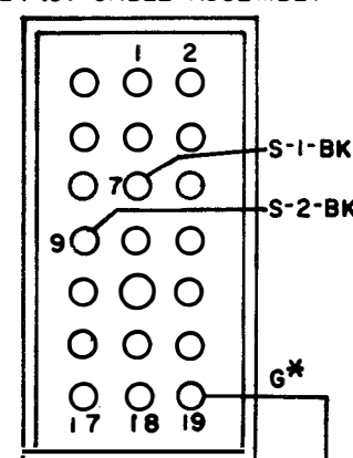
R TYPING UNIT CONNECTOR ON 324497 CABLE ASSEMBLY
