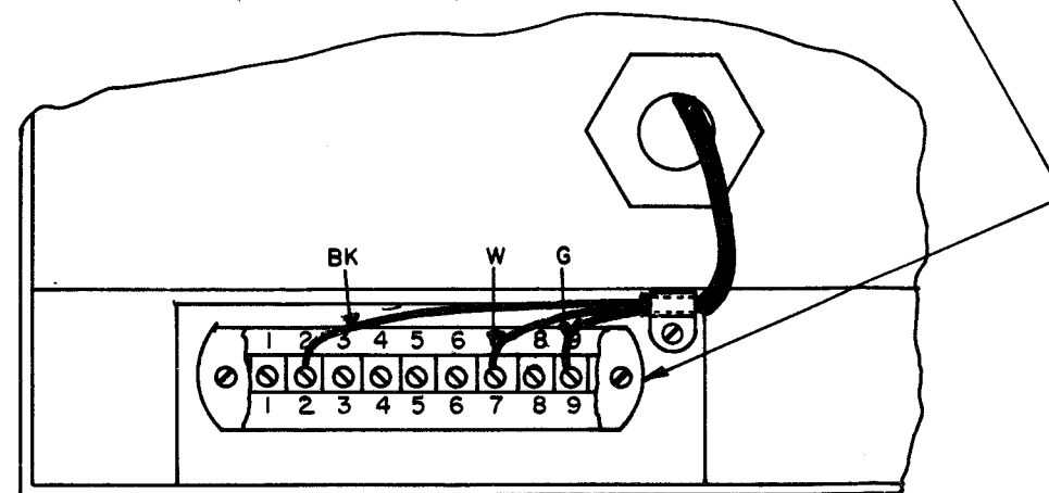
LEFT BOTTOM VIEW (CABLE ROUTING)
