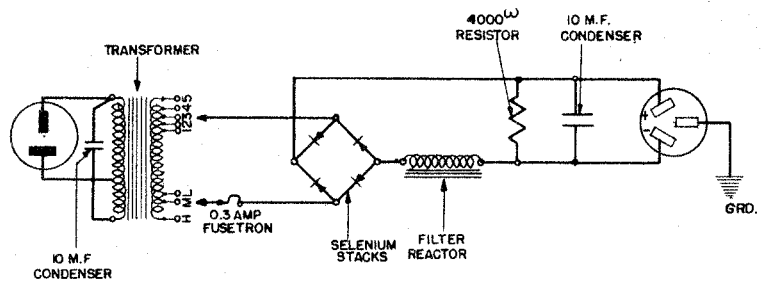
SCHMATIC WIRING
