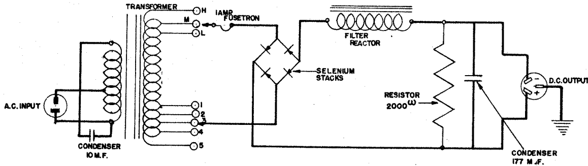
SCHEMATIC
