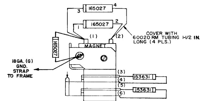
MAGNET WITH 2 NETWORKS AND INTERRUPTER CONTACTS PART OF 193280 STEPPING SWITCH
