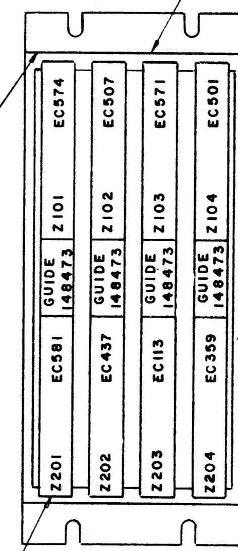
CIRCUIT CARD LOCATION VIEWED FROM WIRE WRAP SIDE.
