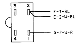
A 158163 MARGIN INDICATOR SWITCH
