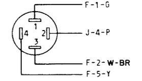
N 304376 SIGNAL LINE BREAK SWITCH
