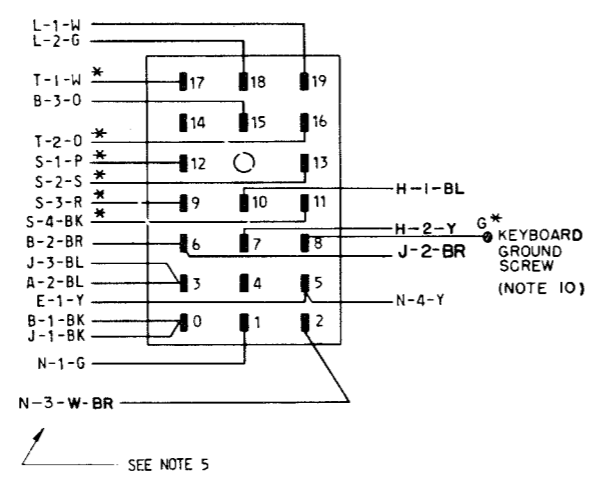
F 152467 KEYBOARD CONNECTOR PLUG
