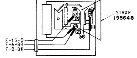
B 197019 CONTACT BOX ASSEMBLY WITH ARC SUPPRESSION NOTE 9
