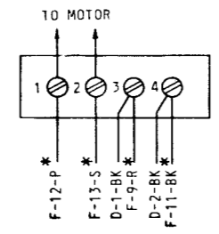
S MOTOR TERMINAL BLOCK
