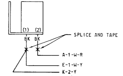
G MARGIN INDICATOR LAMP
