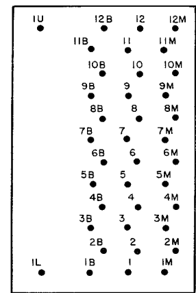
TERMINAL LOCATION 194582 RELAY (AJ12)
