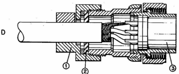
Figure 3-4. Fabrication of Power Cable to A.C. Power Plug P-102
