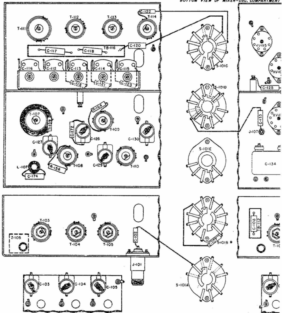
BOTTOM VIEW OF MIXER-DSG. COMPARTMENT
