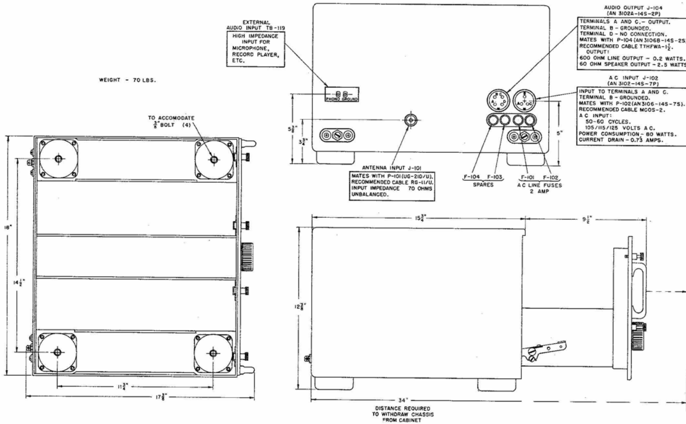
Figure 3-2. Dimensional Outline Drawing
