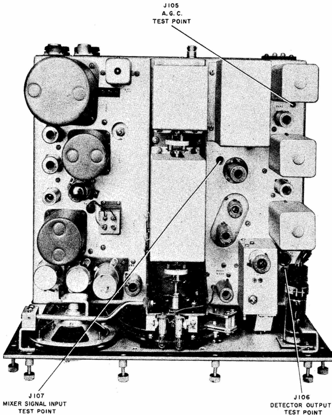
Figure 7-7. Test Point Locations, Top of Chassis
