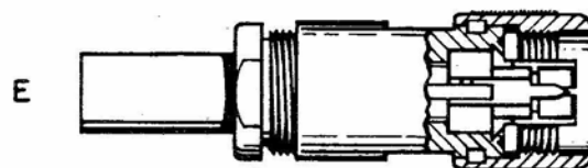
Figure 3-3. Fabrication of Coaxial Cable to Antenna Plug P-101
