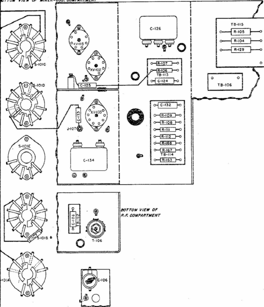
BOTTOM VIEW OF MIXER-OSG. COMPARTMENT
