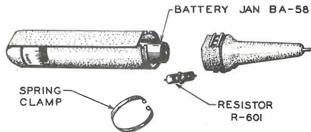
Figure 3-2. Resistance Indicator-Probe, Disassembled
