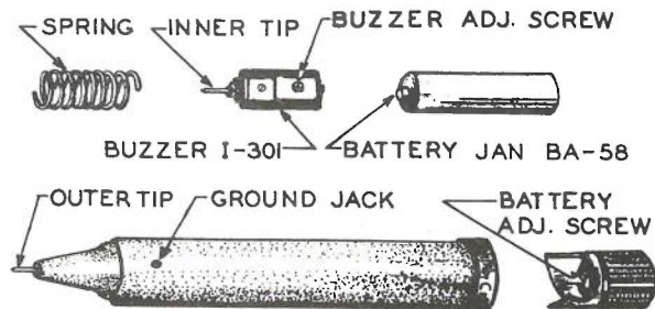
Figure 3-3. Interference Generator, Disassembled
