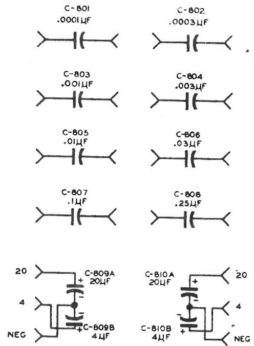
Figure 5-18. Schematic Diagram, Decade Capacitor TS-671/U
