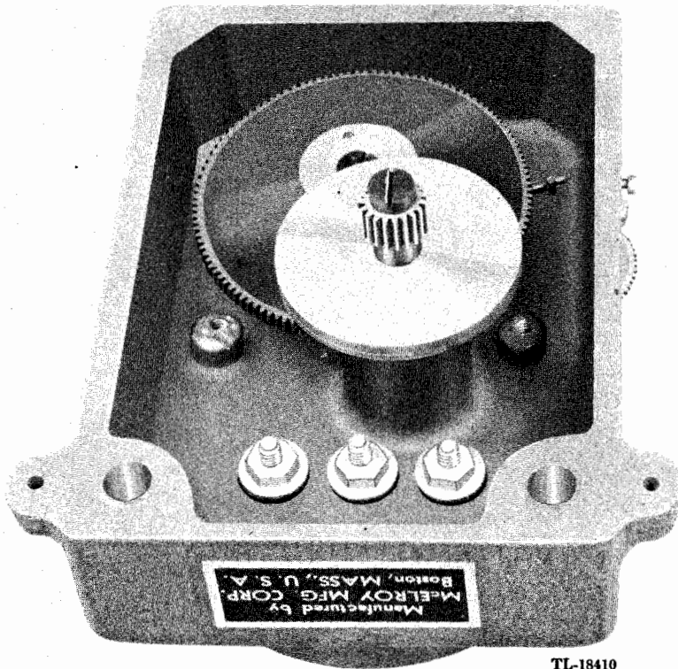
Figure 12. Auto head, rear view.
