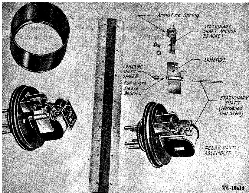
Figure 15. Keying relay.
