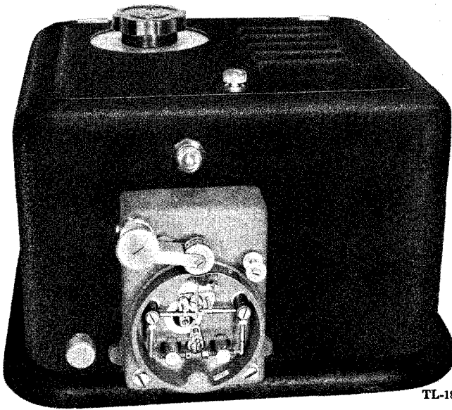
Figure 3. Auto head and drive unit, auto head plate removed.
