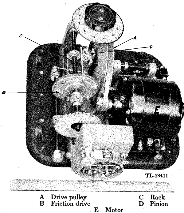
Figure 13. Auto head and drive unit, cover removed.
