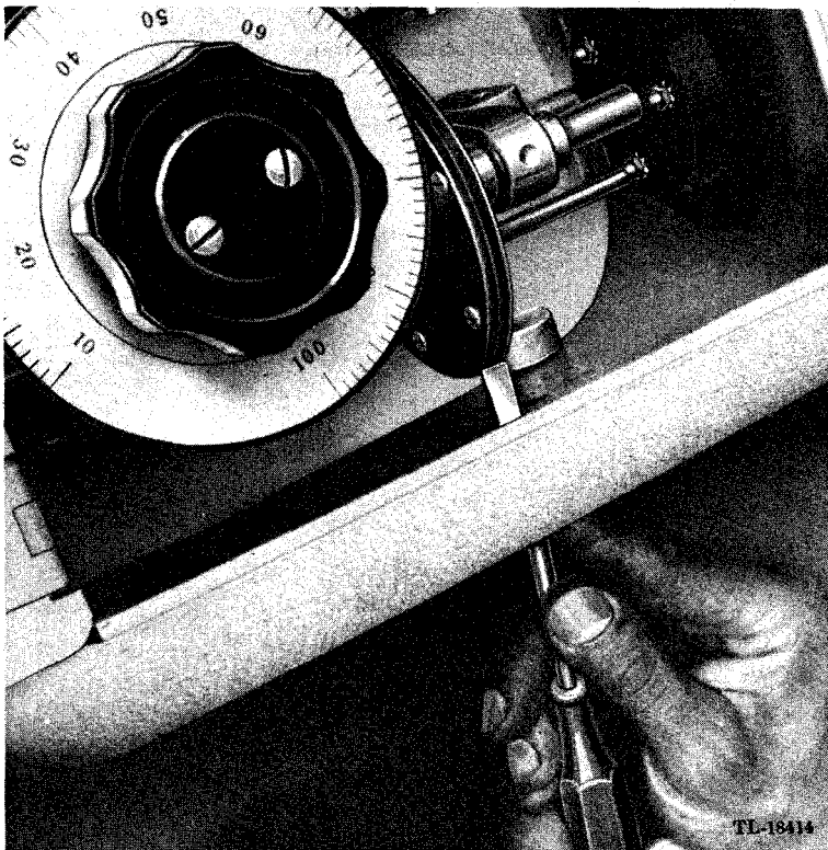
Figure 16. Removing flat from friction-drive disk.
