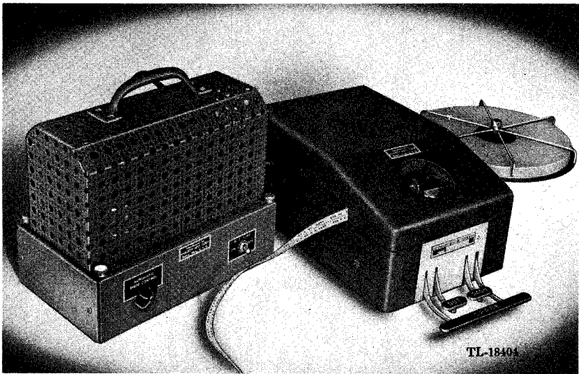
Figure 6. Hand perforator.
