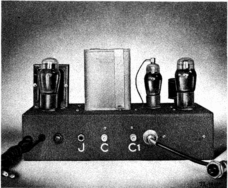
Figure 8. Monitoring jack and tone terminals.
