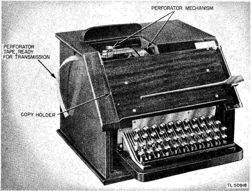
Figure 5. Keyboard perforator.
