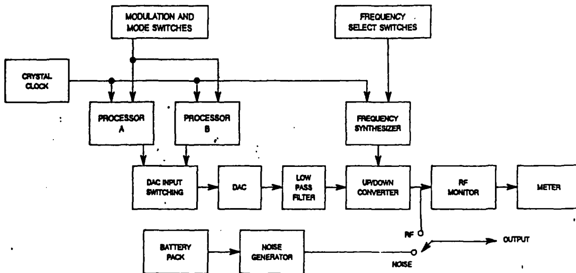
Figure 2. Radio Test Unit Block Diagram
