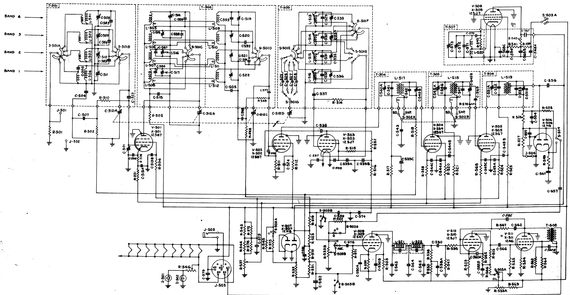
SCHEMATIC DIAGRAM-RBM-5-HF RECEIVER CAY-46077-A
