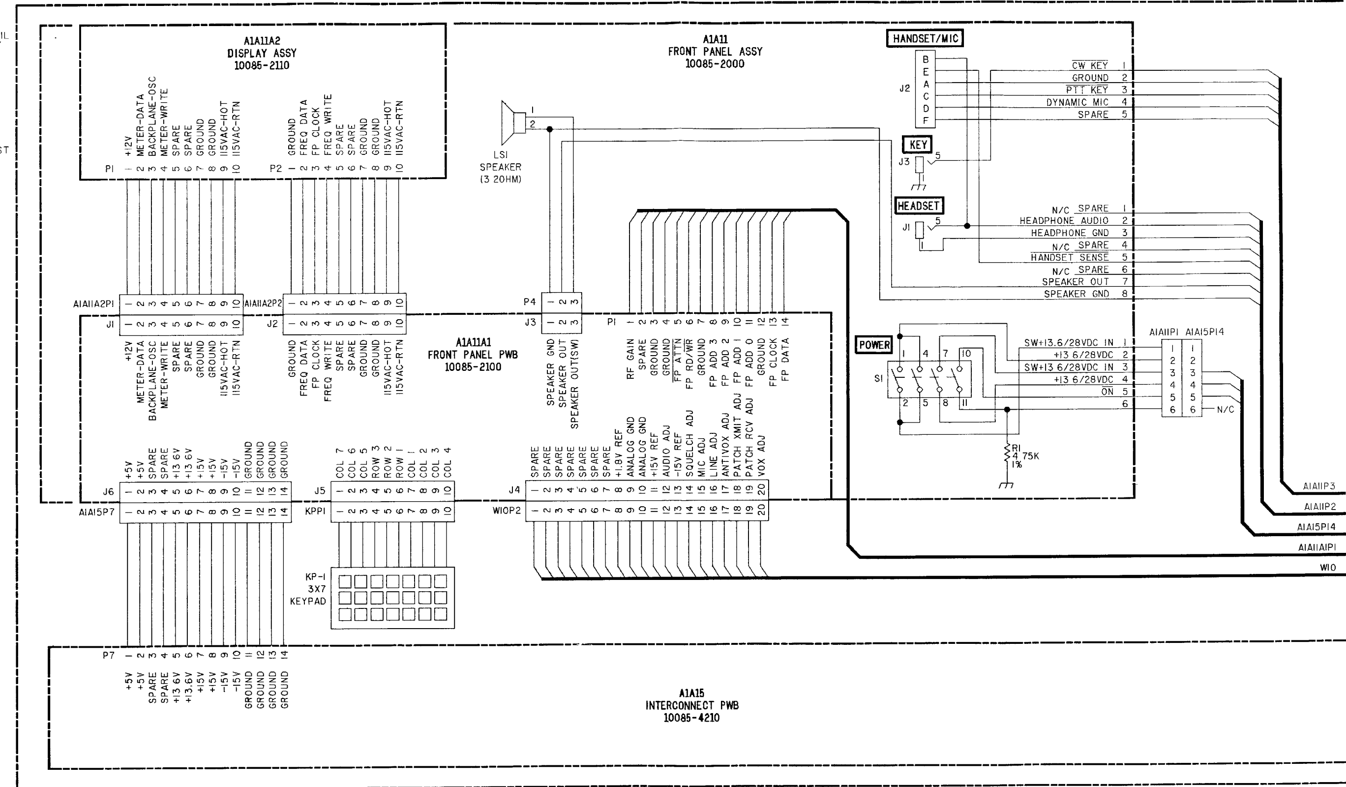
FO-2. TRANSCIVER ASSY, A1, INTERCONNECTION DIAGRAM (Sheet 1 of 13)
