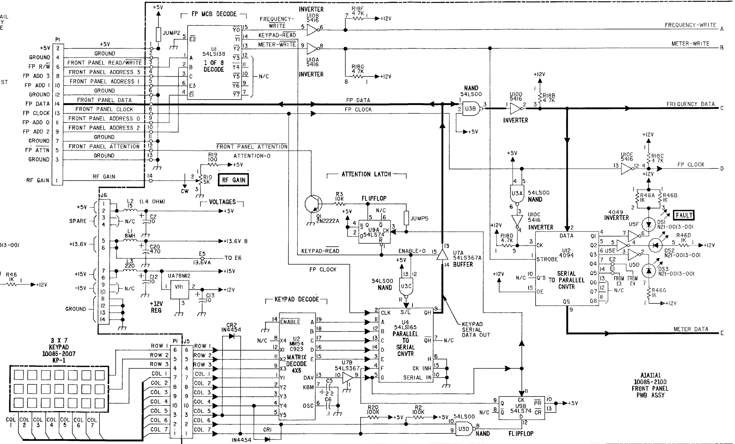
FO-13. FRONT PANEL PWB ASSY, A1A11A1 (Sheet 1 of 2) FP-131/(FP-132 Blank)
