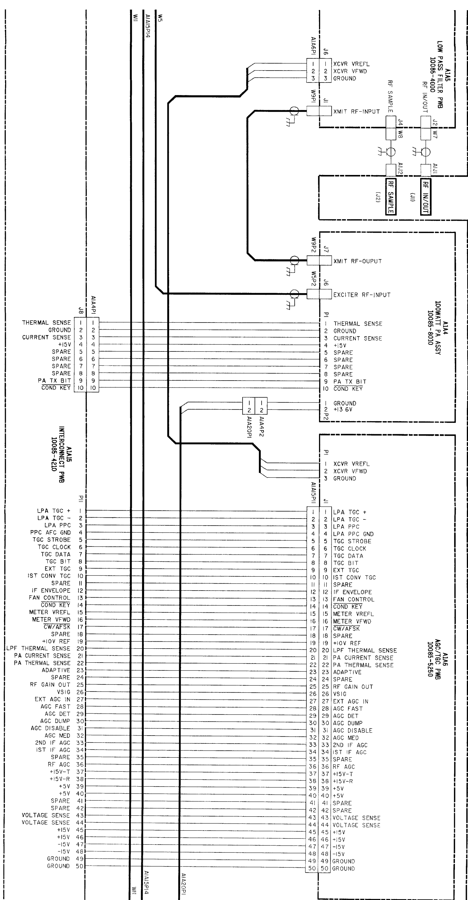
FO-2. TRANSCIVER ASSY, A1, INTERCONNECTION DIAGRAM (Sheet 10 of 13)
