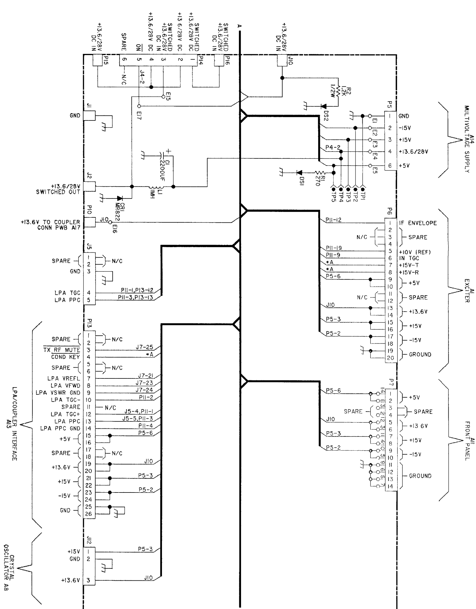
FO-18. INTERCONNECT PWB ASSY, A1A15 (Sheet 2 of 3)
