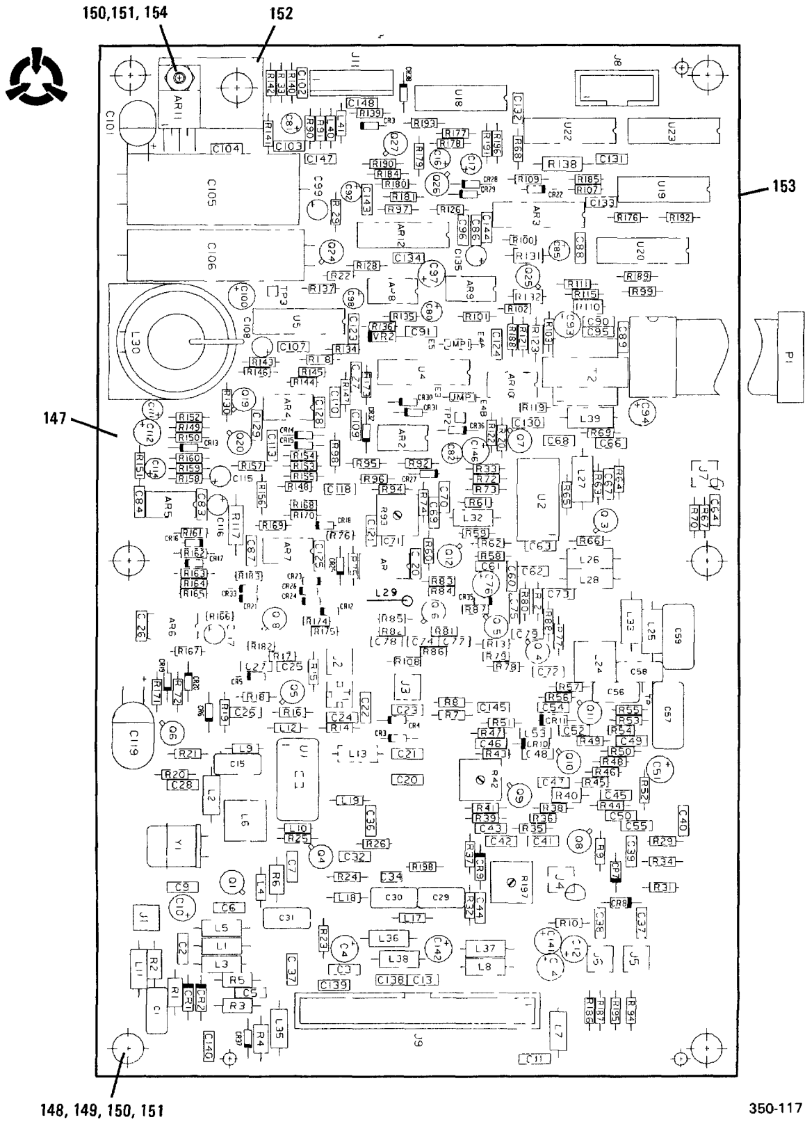
Figure 7-18. Receiver PWB Assy, A1A7
