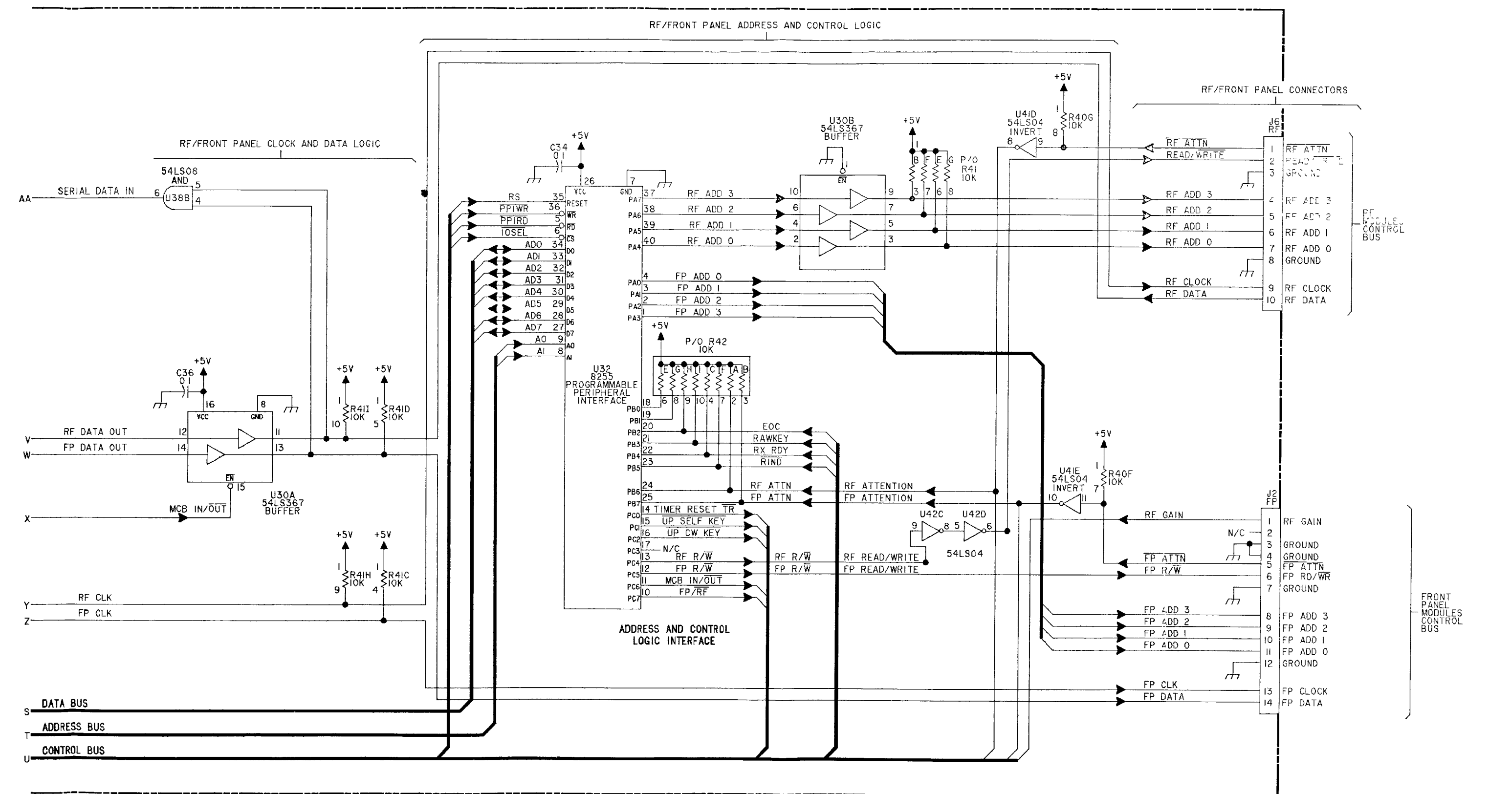
FO-15. TRANSCIVER CONTROL PWB ASSY, A1A12 (Sheet 9 of 9) FP-157/(FP-158 Blank)
